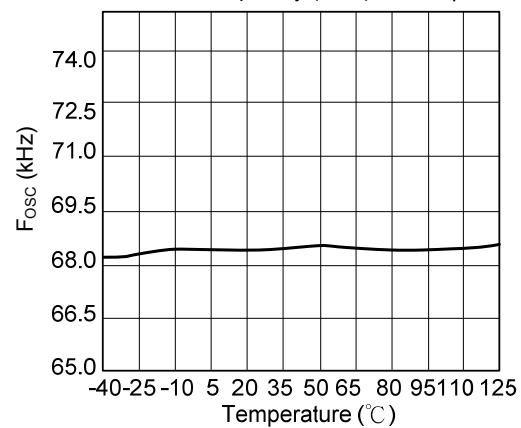
PWM Oscillator Frequency ( F_{OSC} ) vs Temperature
