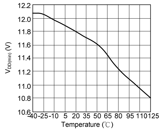
Min. Operating Voltage ( V_{DD(min)} ) vs Temperature
