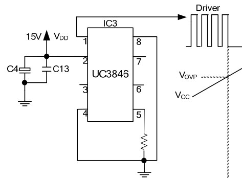
FIG.4 OVP test circuit
