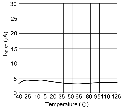
Start-up Current ( I_{DD ST} ) vs Temperature
