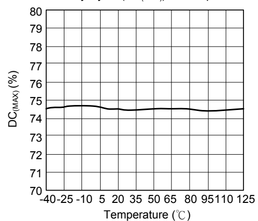
Max. Duty Cycle ( DC_{(MAX)} ) vs Temperature
