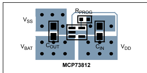
FIGURE 6-4: Typical Layout (Top).
