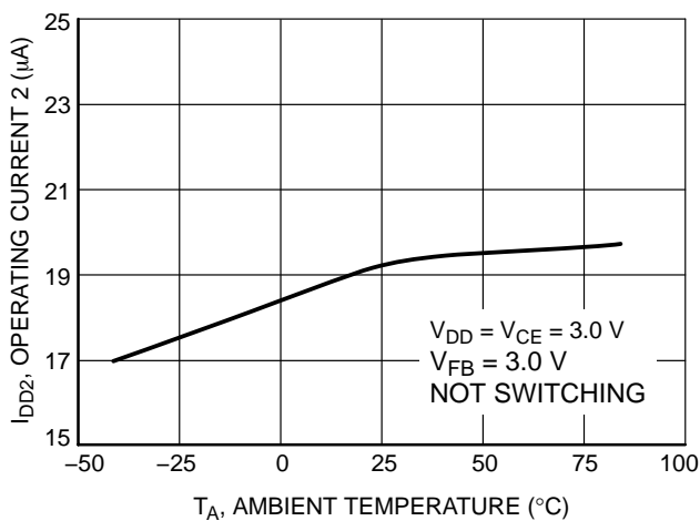
Figure 19. Operating Current 2 versus Ambient Temperature
