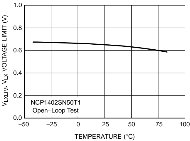
Figure 29. NCP1402SN50T1 V LX Voltage Limit vs. Temperature
