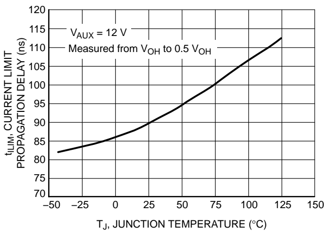
Figure 13. Current Limit Propagation Delay versus Junction Temperature
