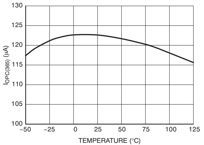
Figure 14. Maximum Overpower Compensating Current I_{OPC(365)} Flowing Out of CS Pin
