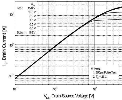
Figure 1. Output Characteristics
