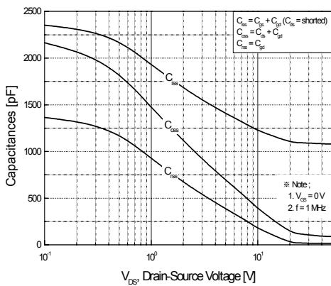
Figure 5. Capacitance vs. Drain-Source Voltage
