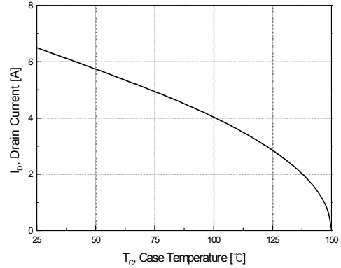
Figure 10. Max. Drain Current vs. Case Temperature
