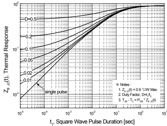
Figure 11. Thermal Response
