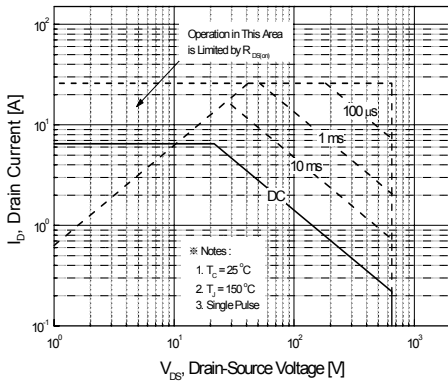
Figure 9. Max. Safe Operating Area
