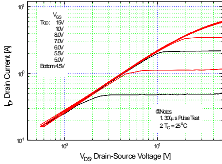
Figure 1. Output Characteristics
