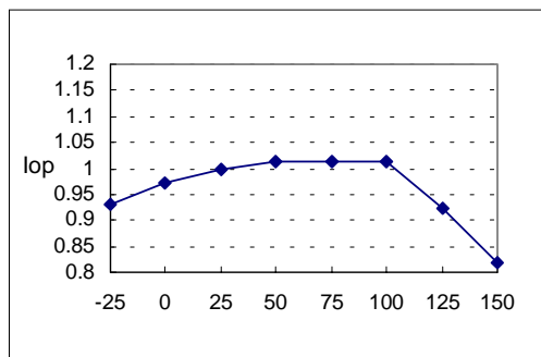
Figure 3. Operating Current
