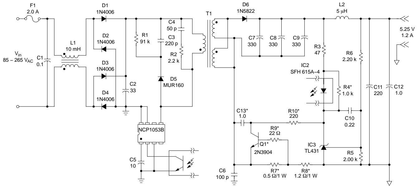
Figure 28. Universal Input 6/5 Watt Converter/Charger Application
