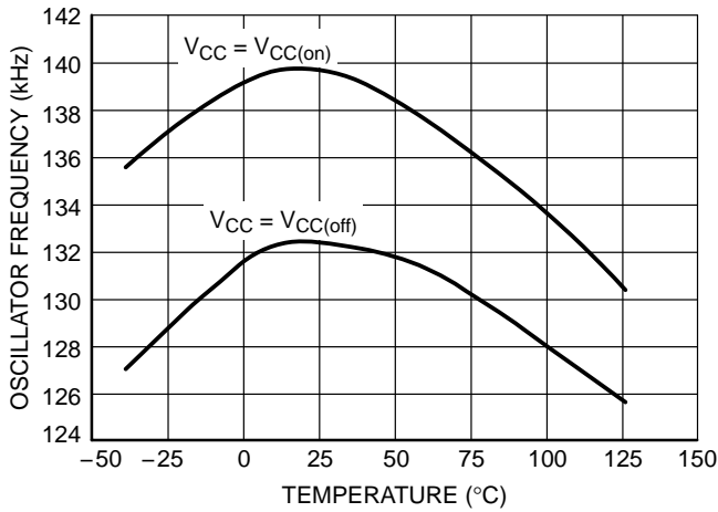
Figure 7. Oscillator Frequency (C Suffix) versus Temperature
