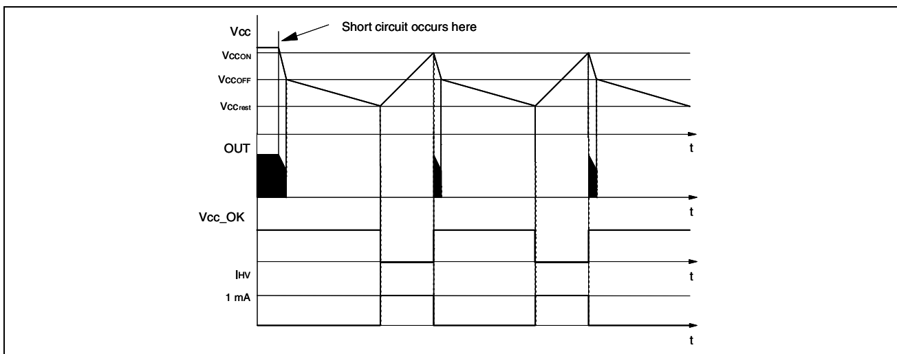
Figure 37. Timing diagram showing short-circuit behavior
