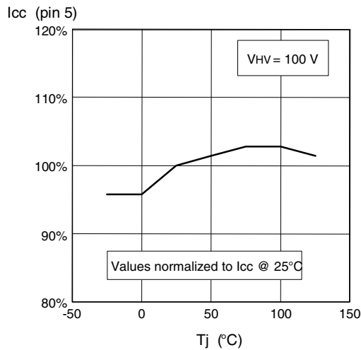
Figure 7. High-voltage pin leakage vs. Tj
