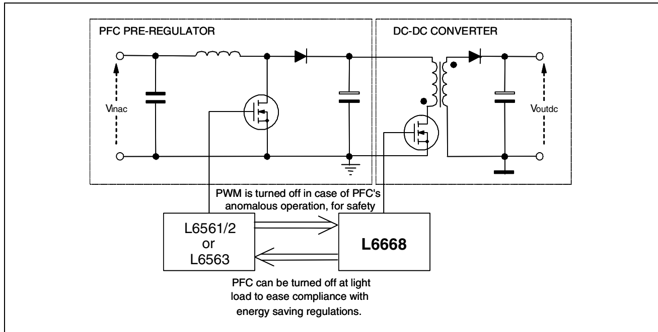
Figure 4. Typical System Block Diagram
