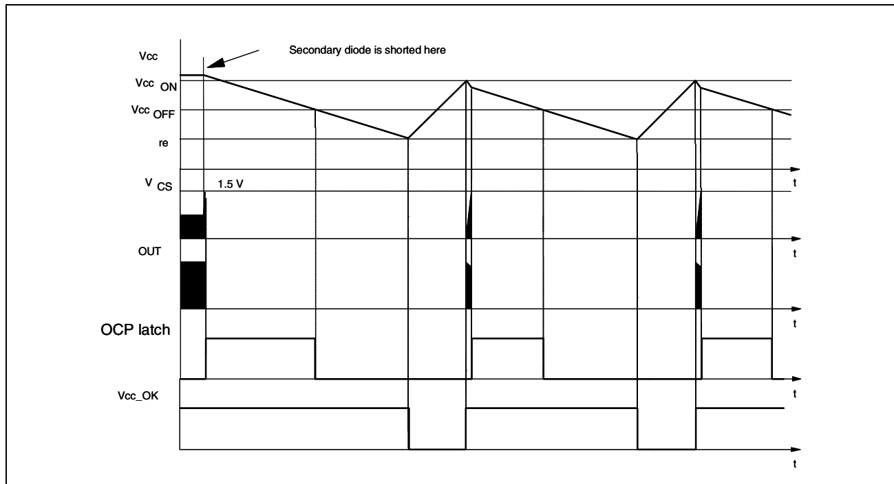
Figure 41. Hiccup-mode OCP: timing diagram
