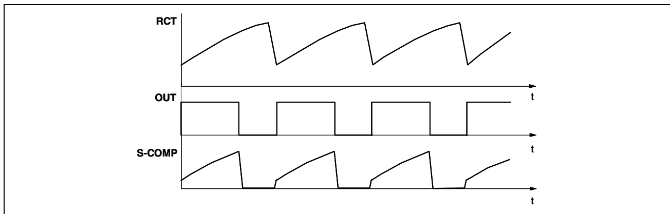
Figure 45. Slope compensation waveforms
