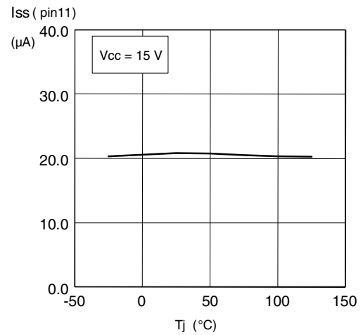
Figure 28. Soft-start charge current vs. Tj
