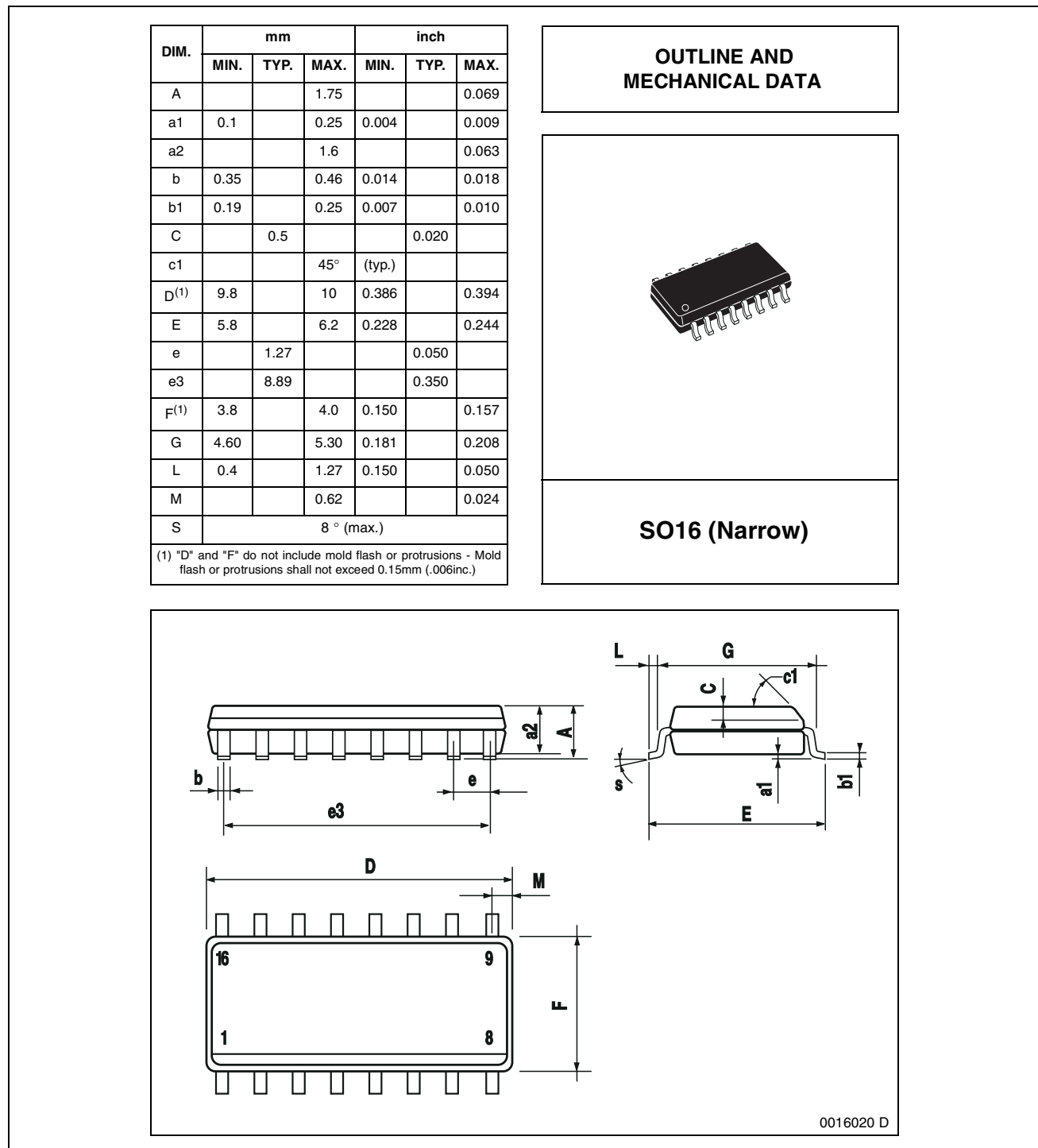
Figure 47. SO16 (Narrow) Mechanical Data & Package Dimensions
