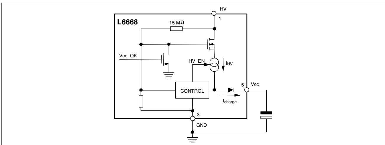
Figure 35. High-voltage start-up generator: internal schematic
