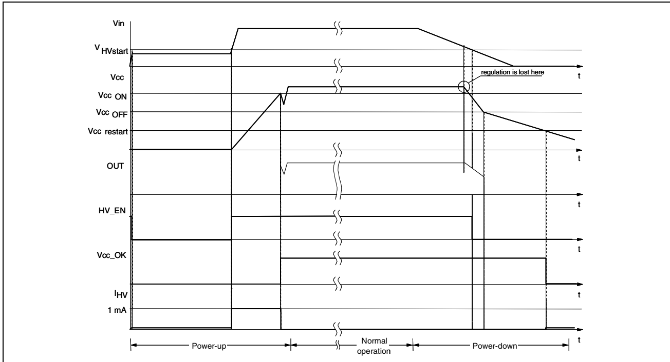
Figure 36. Timing diagram: normal power-up and power-down sequences
