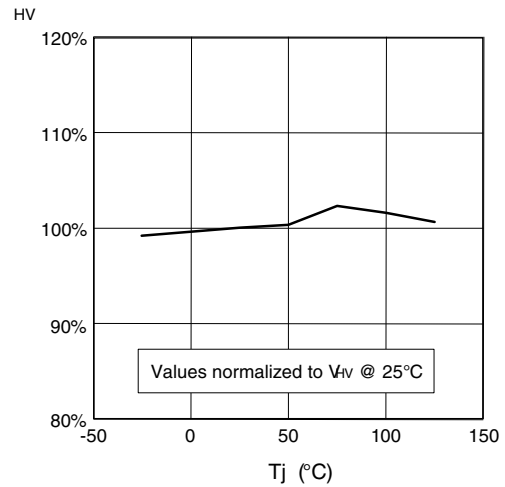
Figure 9. High-voltage generator Vcc restart voltage vs. Tj
