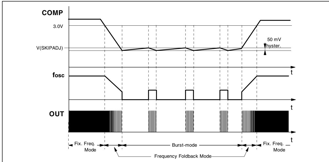
Figure 40. Load-dependent operating modes: timing diagram
