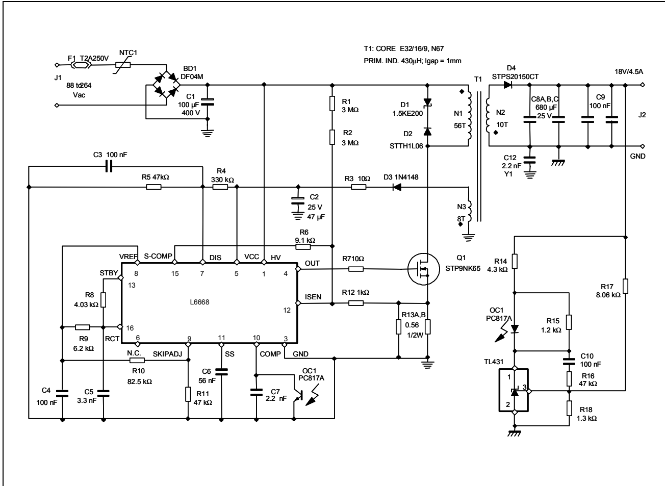
Figure 46. Typical Application: 80W, WRM flyback; Electrical Schematic
