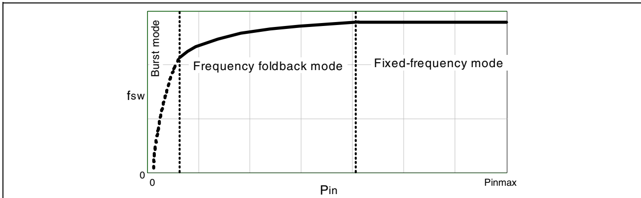
Figure 34. Multi-mode operation of the L6668
