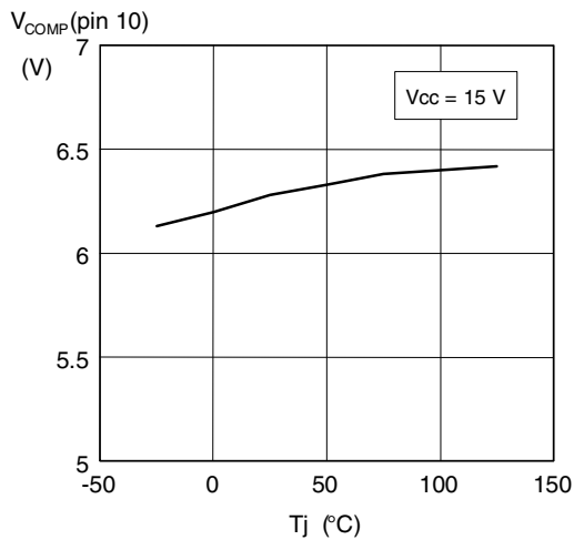
Figure 13. COMP voltage upper clamp level vs. Tj
