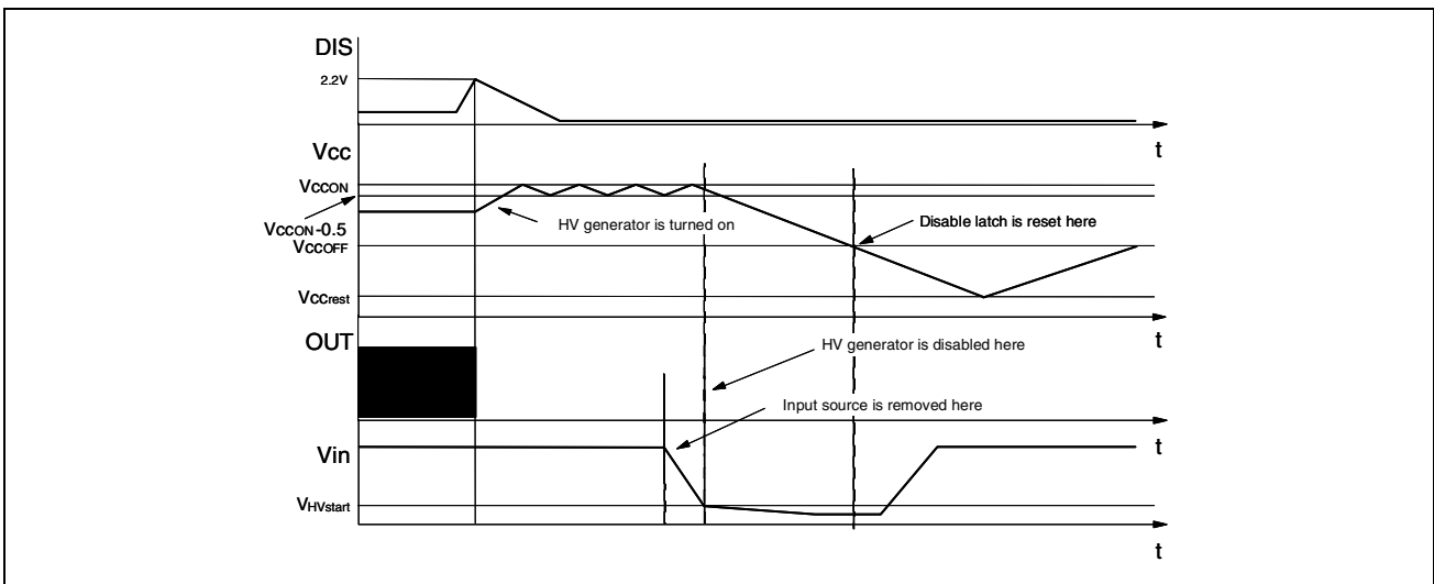
Figure 44. Operation after DIS pin activation: timing diagram
