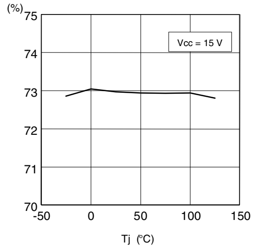
Figure 16. Max. duty-cycle vs. Tj
