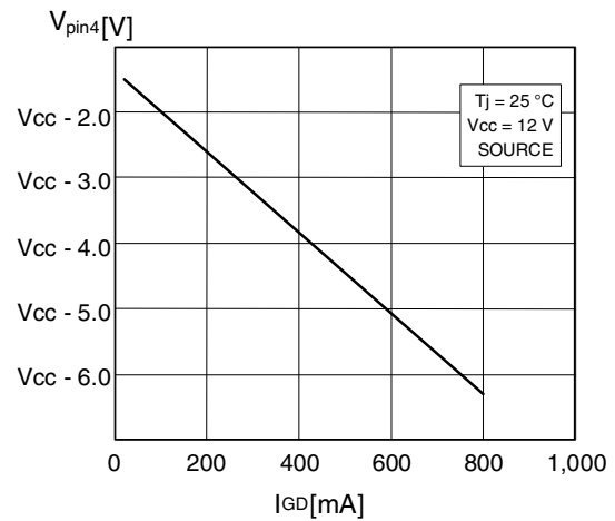
Figure 33. Gate-drive output high saturation
