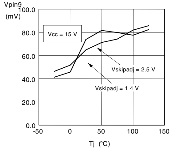
Figure 27. SKIPADJ disable threshold vs. Tj
