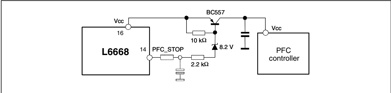
Figure 43. Operation of PFC_STOP function
