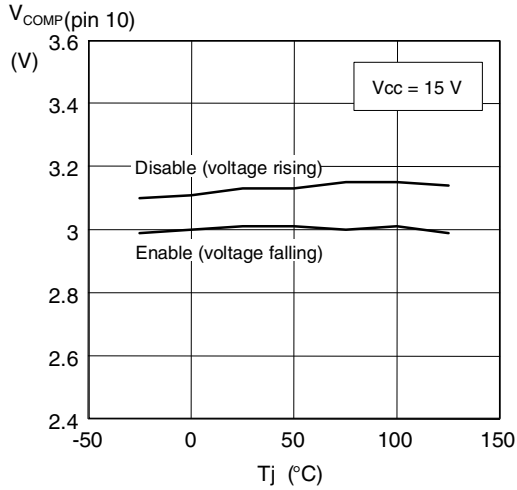
Figure 24. Standby pin dropout vs. Tj
