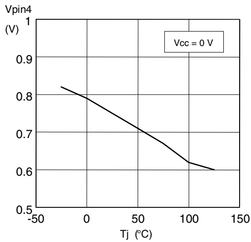
Figure 31. Gate-drive clamp vs. Tj
