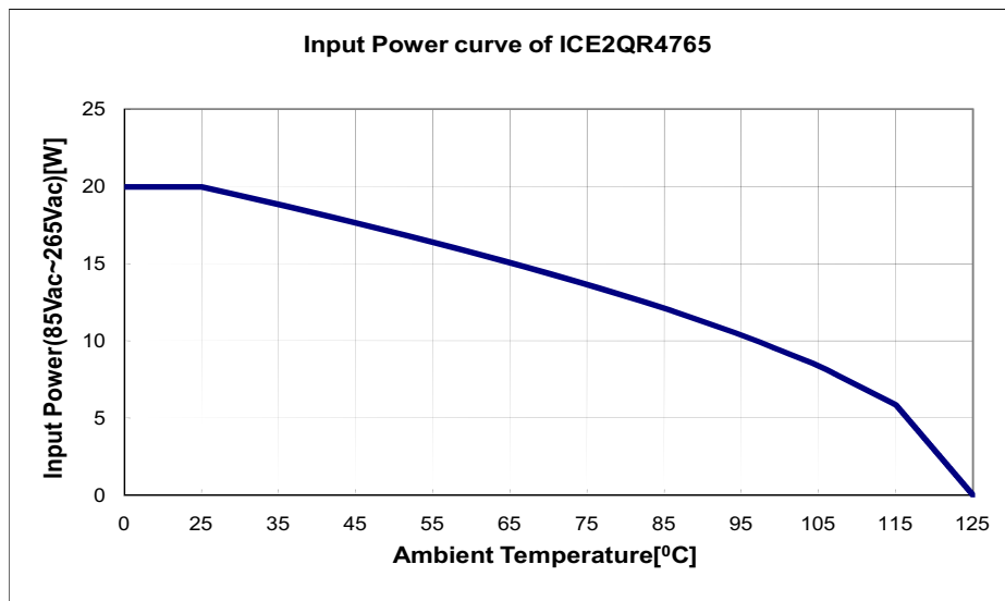
Figure 12 Input Power curve V_{in}=85\sim 265\text{Vac}; P_{in}=f(T_a)
