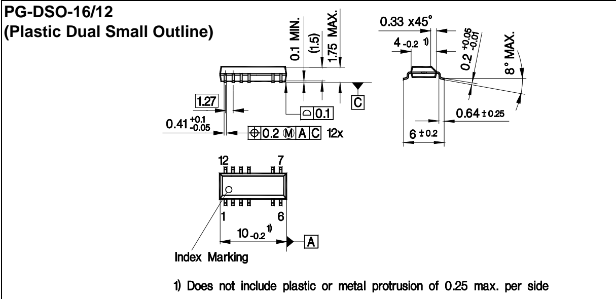
Figure 14 PG-DSO-16/12 (Pb-free lead plating Plastic Dual Small Outline Package)
