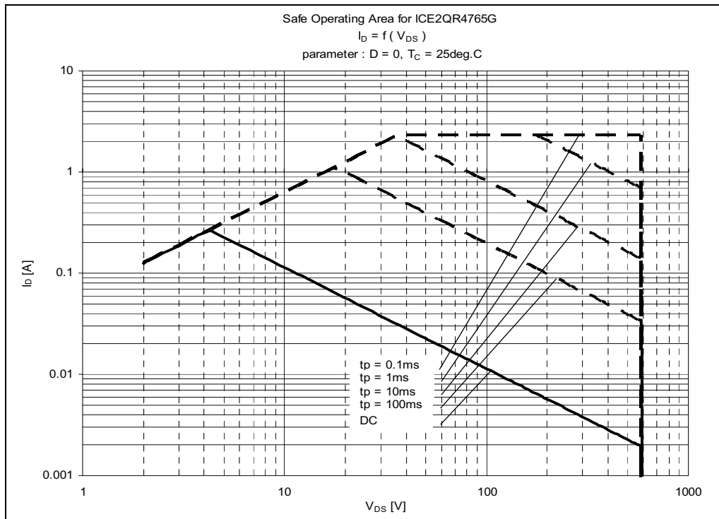
Figure 9 Safe Operating Area(SOA) curve for ICE2QR4765G
