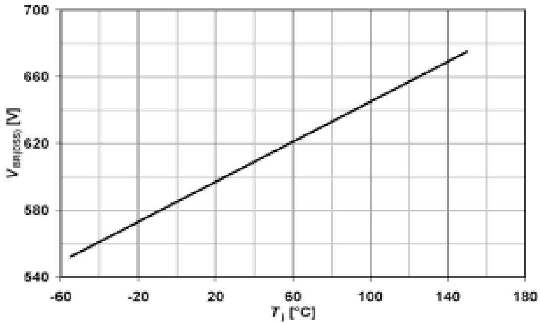
Figure 11 Drain-source breakdown voltage; V_{BR(DSS)}=f(T_j)
