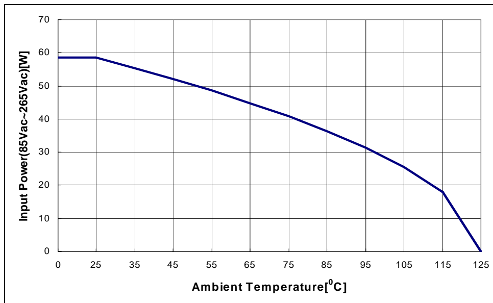
Figure 12 Input Power curve V_{in}=85\sim 265\text{Vac}; P_{in}=f(T_a)
