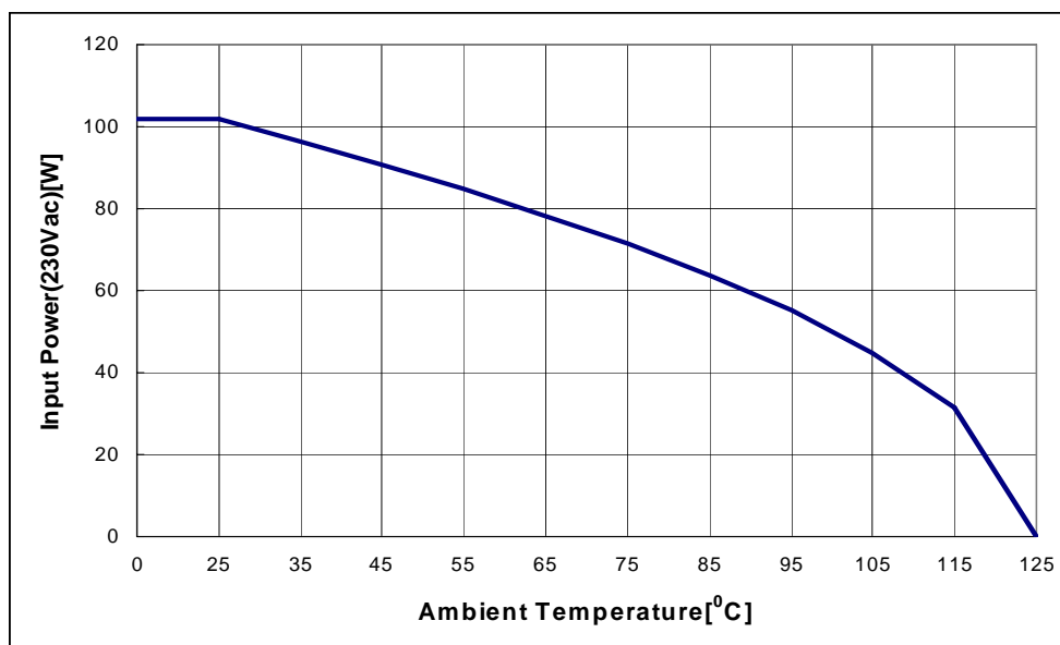
Figure 13 Input Power curve V_{in}=230\text{Vac}; P_{in}=f(T_a)
