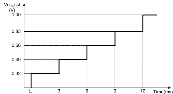
Figure 4 Maximum current sense voltage during softstart
