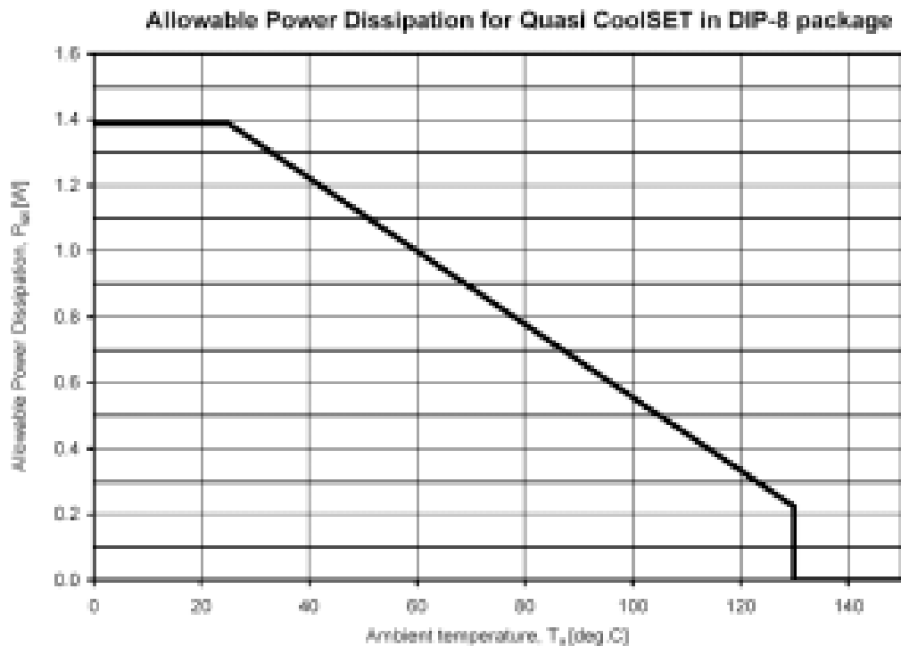
Figure 10 Power dissipation; P_{tot}=f(T_a)
