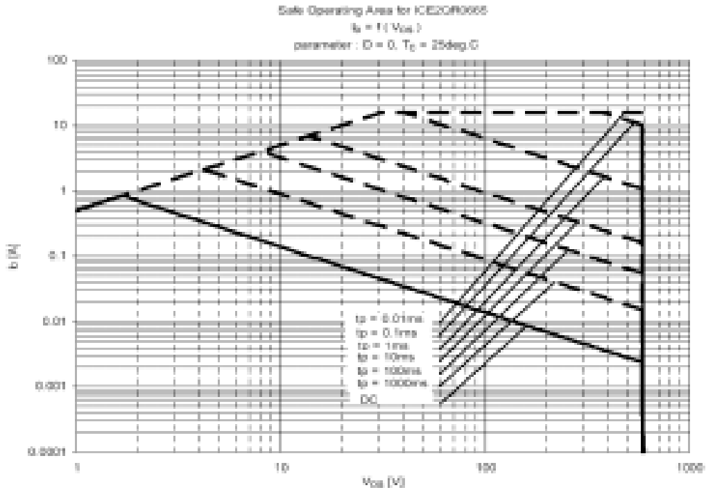
Figure 9 Safe Operating Area(SOA) curve for ICE2QR0665
