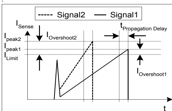
Figure 14 Current Limiting
