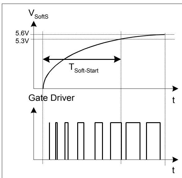
Figure 9 Soft-Start Phase
