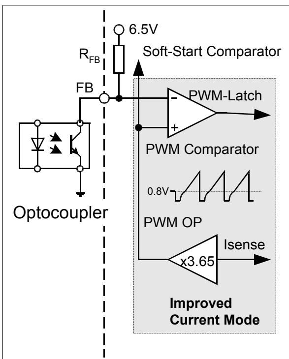
Figure 8 PWM Controlling
