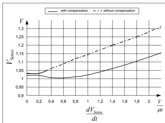
Figure 16 Overcurrent Shutdown
