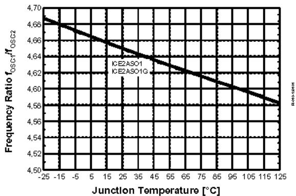
Figure 34 Frequency Ratio f_{OSC1} / f_{OSC2} vs. T_J
