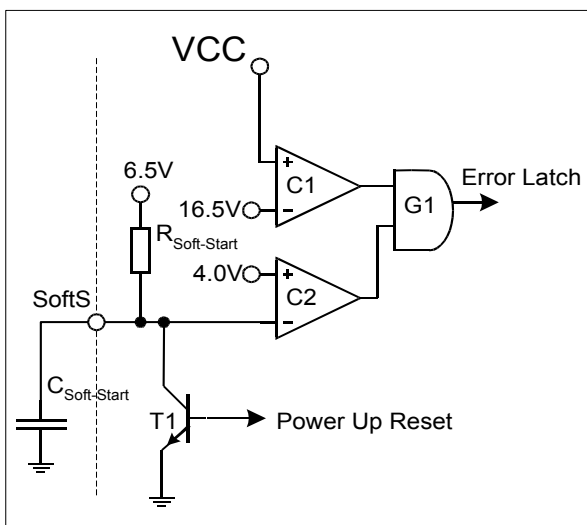
Figure 22 Overvoltage Detection
