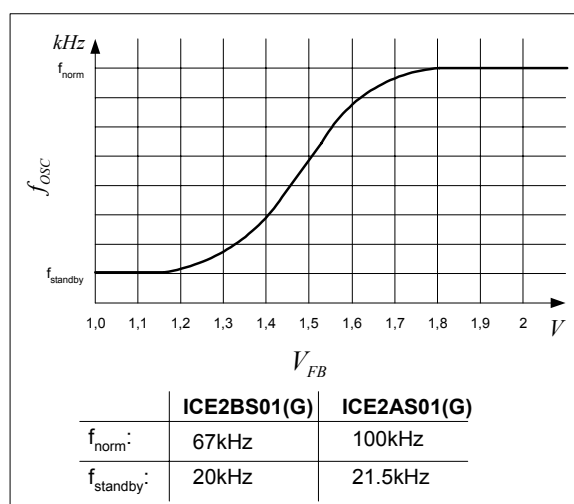
Figure 12 Frequency Dependence
