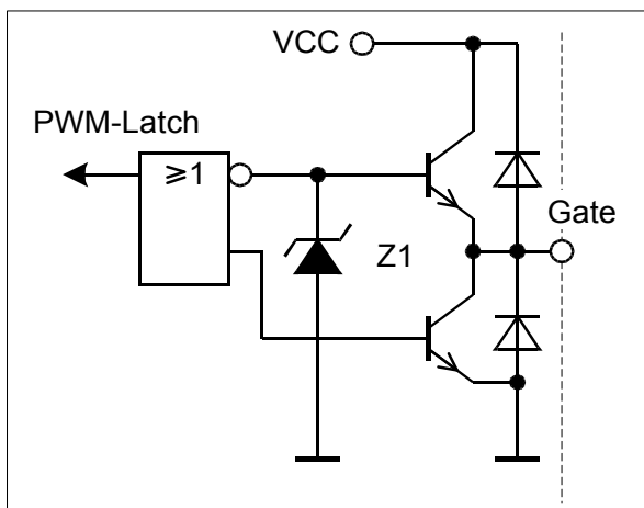
Figure 17 Gate Driver
