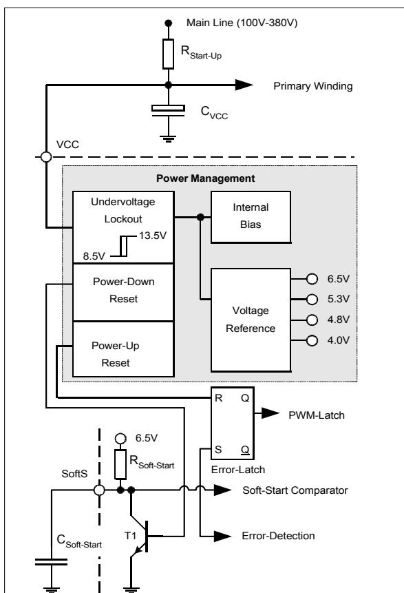
Figure 3 Power Management
