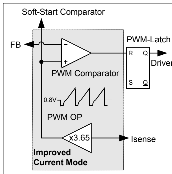
Figure 4 Current Mode
