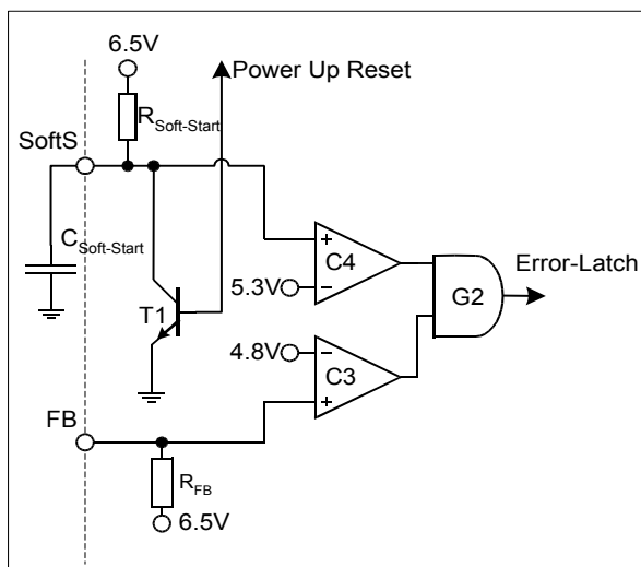
Figure 20 FB-Detection
