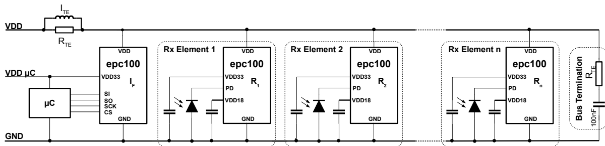
Figure 4: Typical light curtain receiver edge circuit
