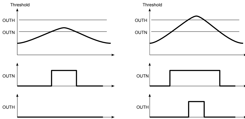
Figure 2: OUTH and OUTN threshold operation
