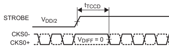
Figure 19. Serializer Clock Propagation Delay
