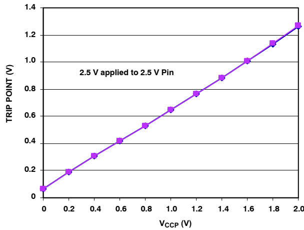
Figure 12. \overline{THERM} Input Threshold vs. V_{CCP} Voltage
