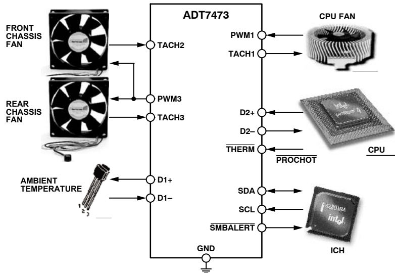
Figure 12. ADT7473 Configuration
