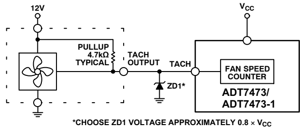
Figure 41. Fan with TACH Pullup to Voltage > 3.6 V Clamped with Zener Diode
