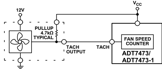
Figure 40. Fan with TACH Pullup to V CC
