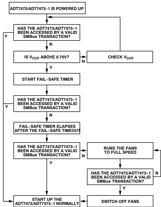
Figure 46. Power-On Flow Chart
