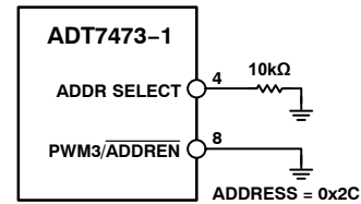
Figure 14. SMBus Address = 0x2C (Pin4 = 0)
