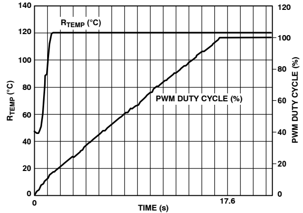
Figure 79. Enhanced Acoustics Mode with Ramp Rate = 2
