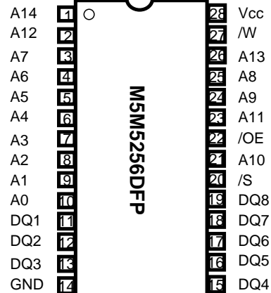
Outline 28P2W-C (DFP)
