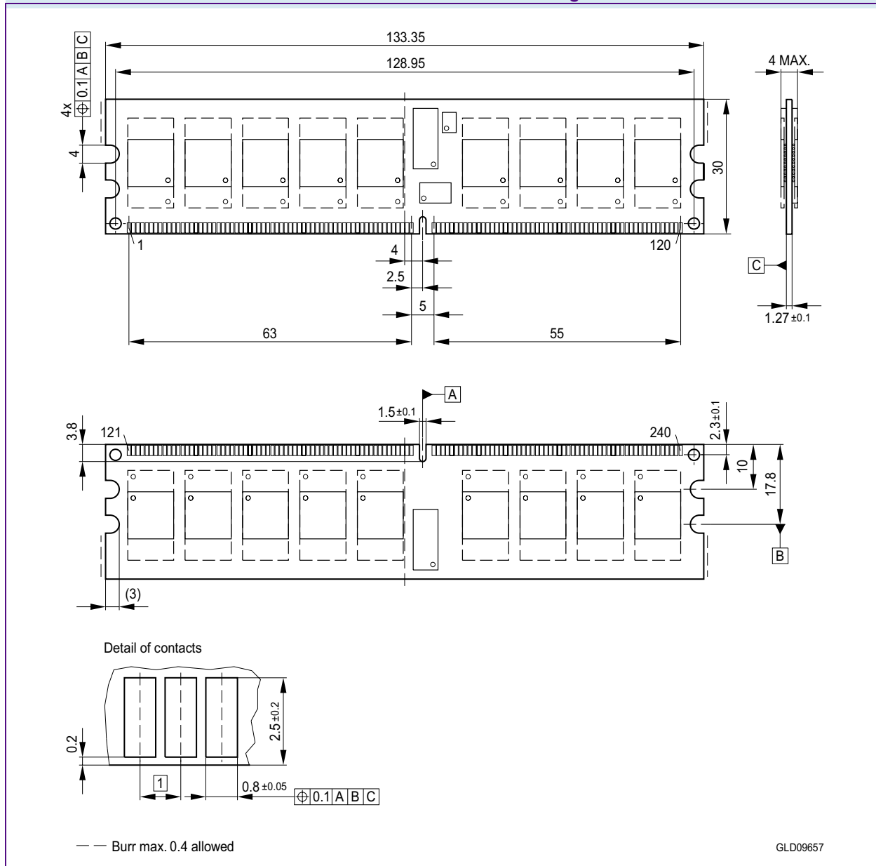
FIGURE 6 Package Outline Raw Card H L-DIM-240-13
