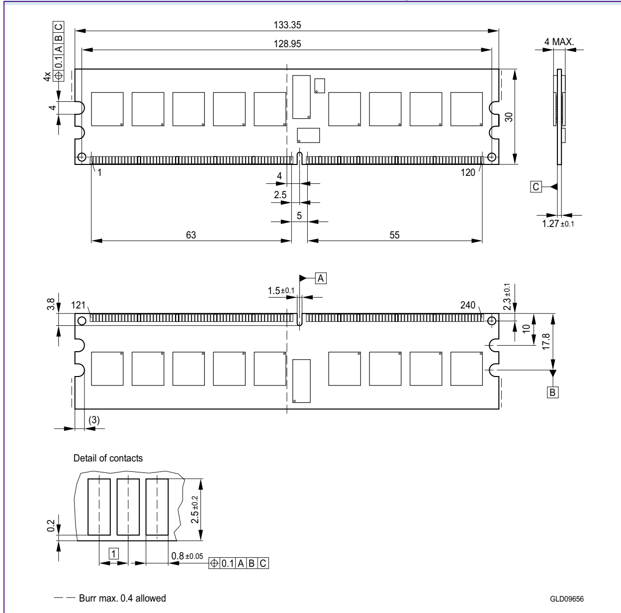
FIGURE 7 Package Outline Raw Card G L-DIM-240-12
