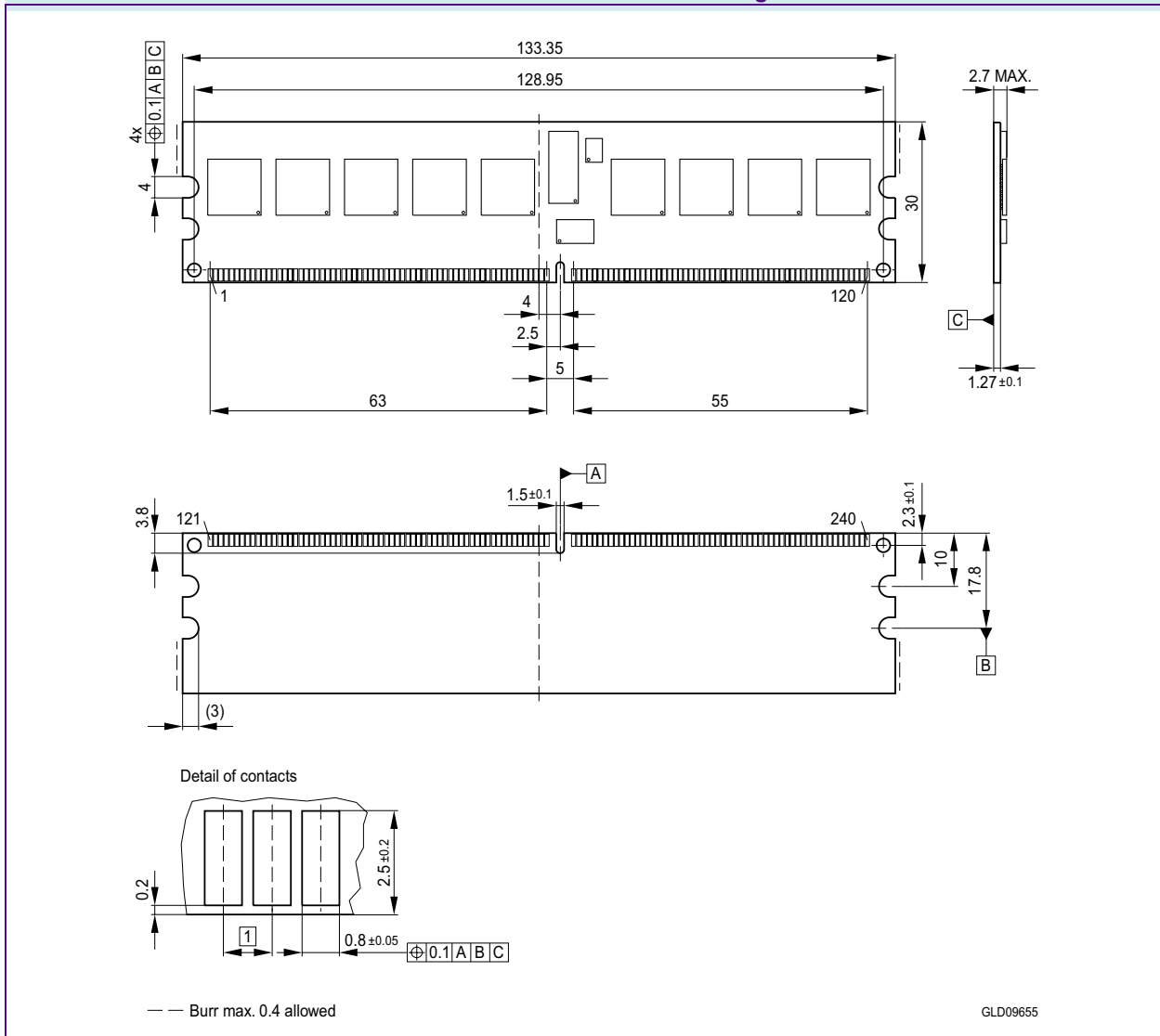
FIGURE 5 Package Outline Raw Card F L-DIM-240-11
