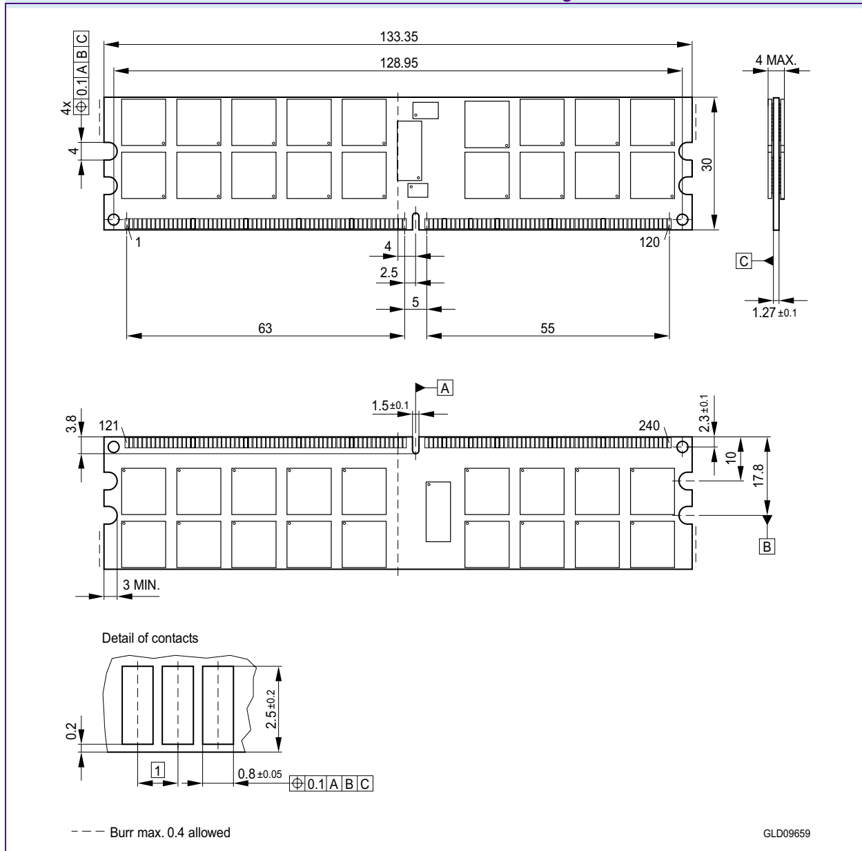
FIGURE 9 Package Outline Raw Card L L-DIM-240-48
