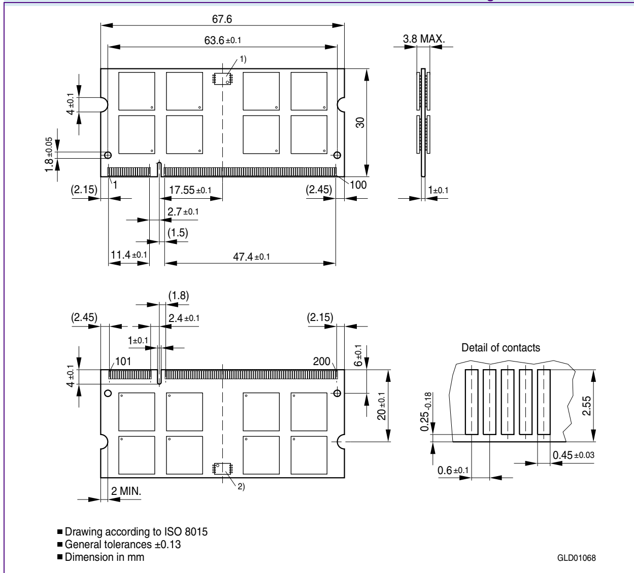
FIGURE 7 Package Outline L-DIM-200-36
