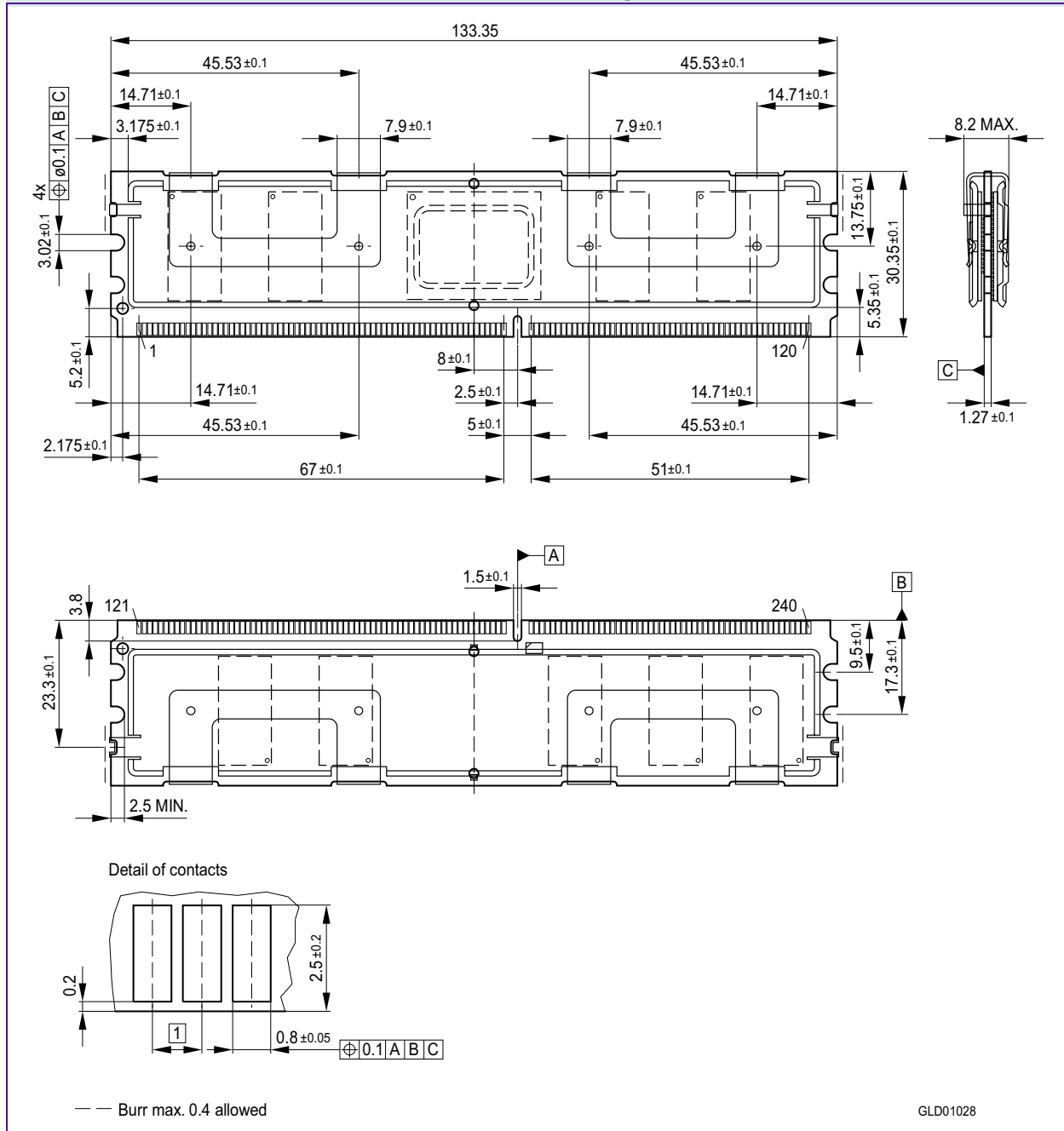
Package Outline L-DIM-240-21 with Full Heat Sink
