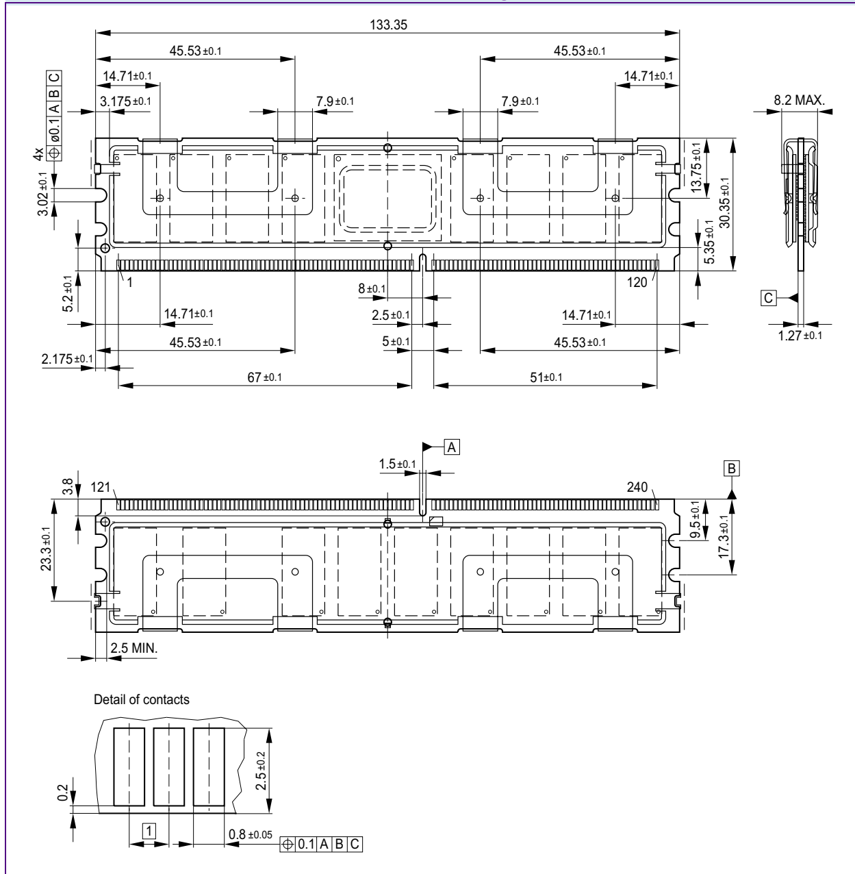
FIGURE 5 Package Outline L-DIM-240-22 with Full Heat Sink
