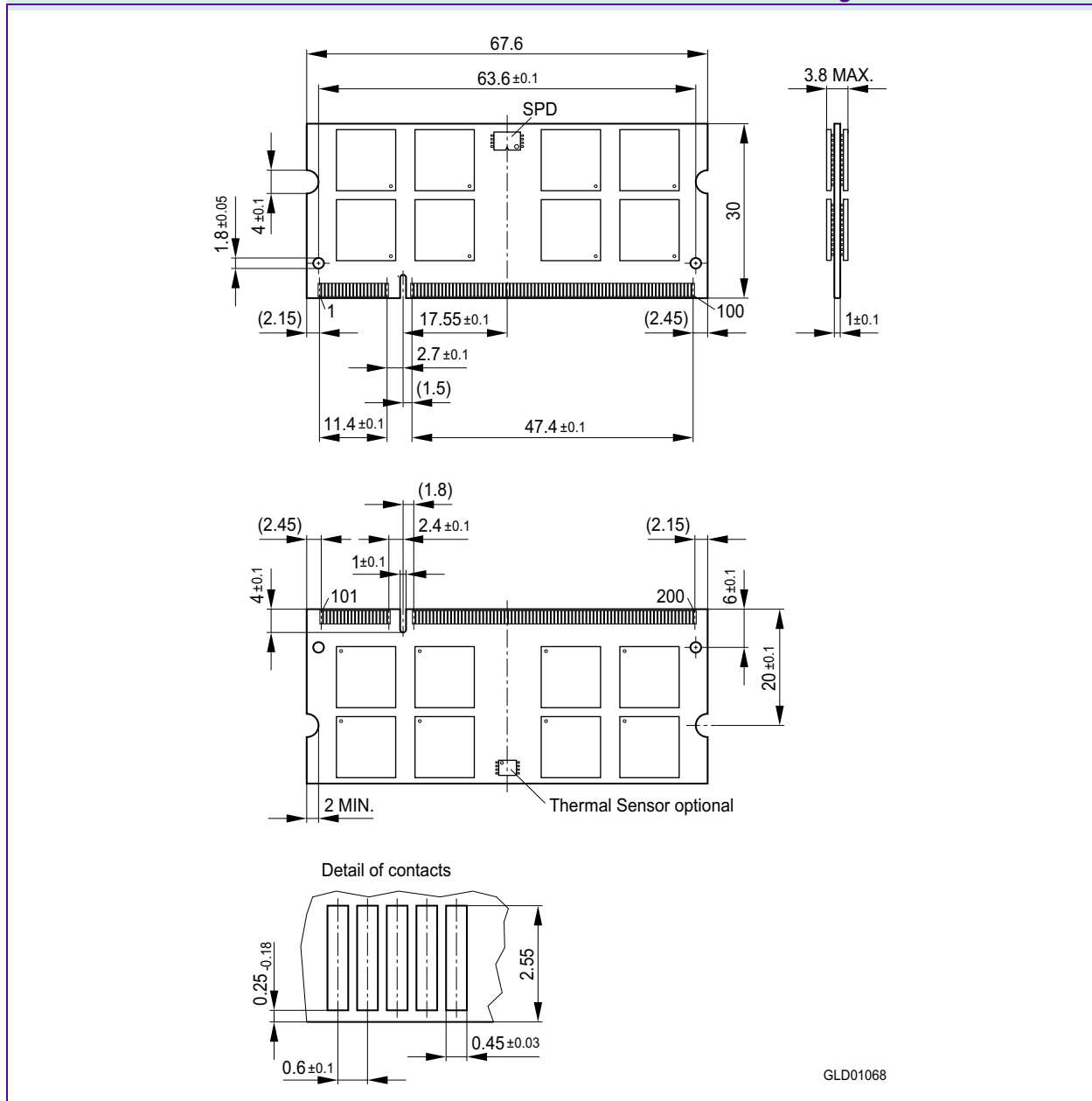
FIGURE 7 Package Outline L-DIM-200-36
