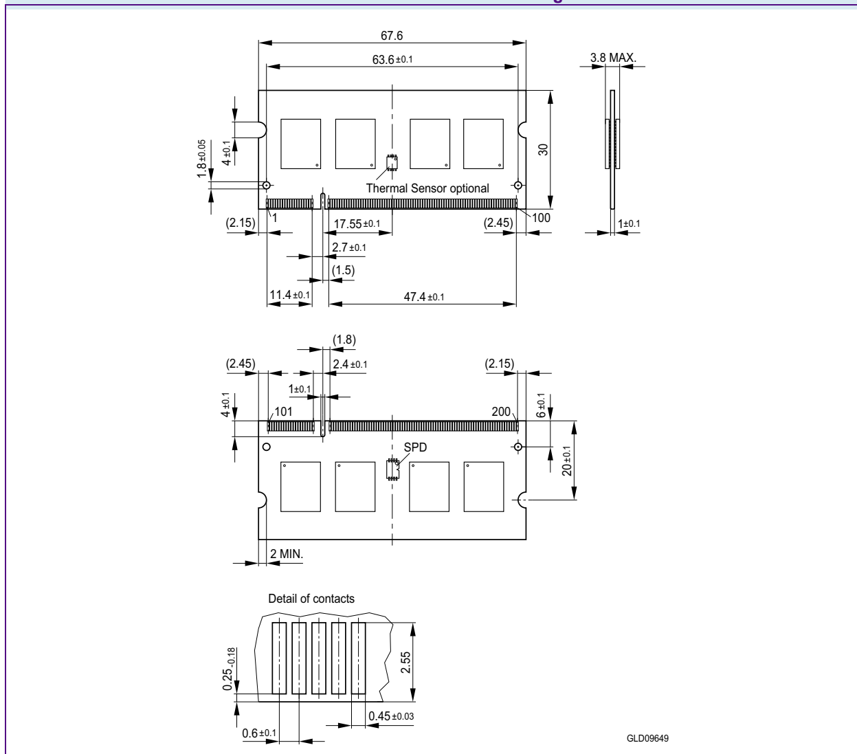
FIGURE 5 Package Outline Raw Card A L-DIM-200-31
