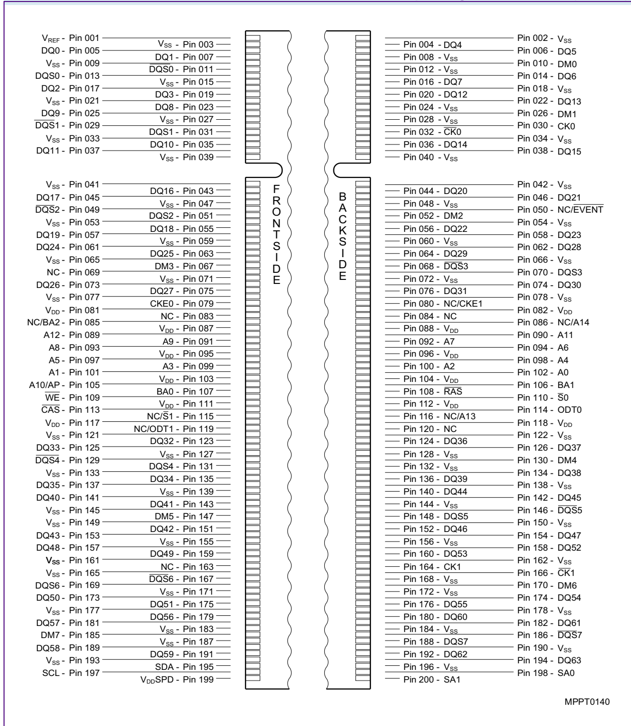
FIGURE 1 Chip Configuration SO-DIMM (200 Ball)
