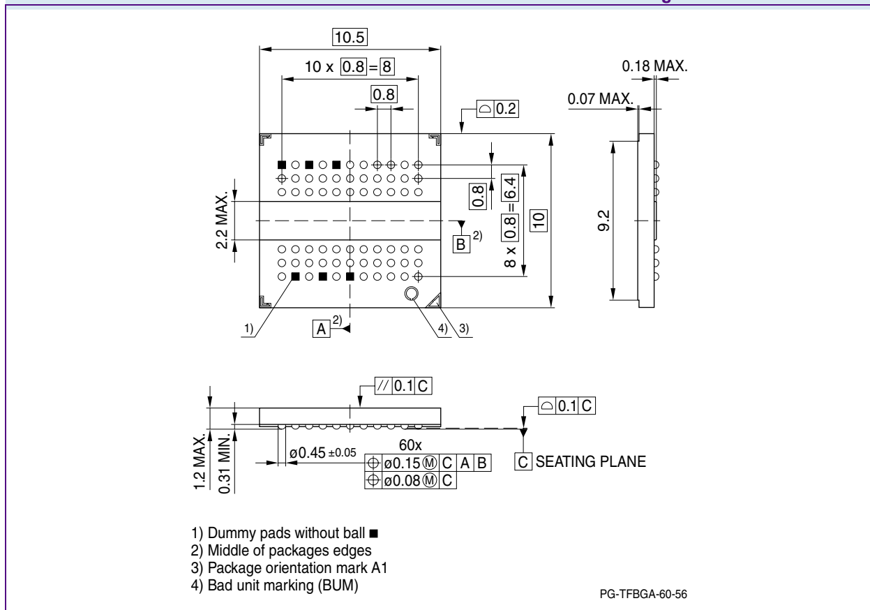
FIGURE 11 Package Outline PG-TFBGA-60
