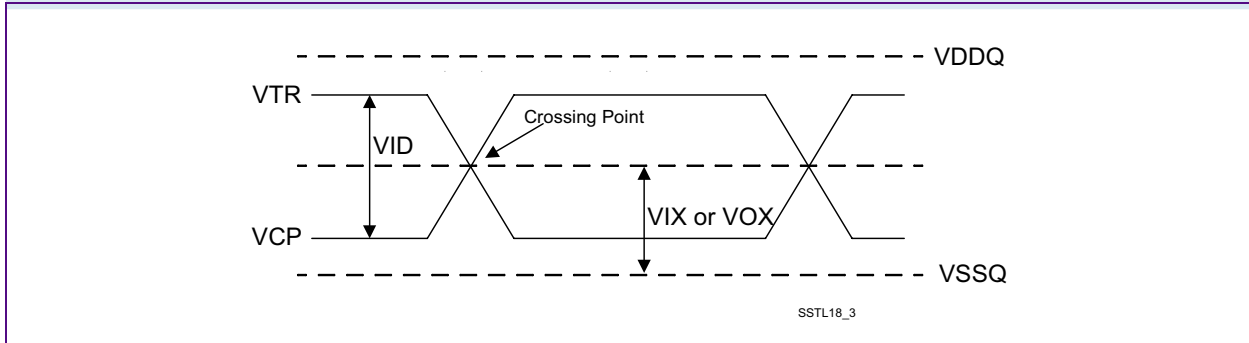
FIGURE 5 Differential DC and AC Input and Output Logic Levels Diagram
