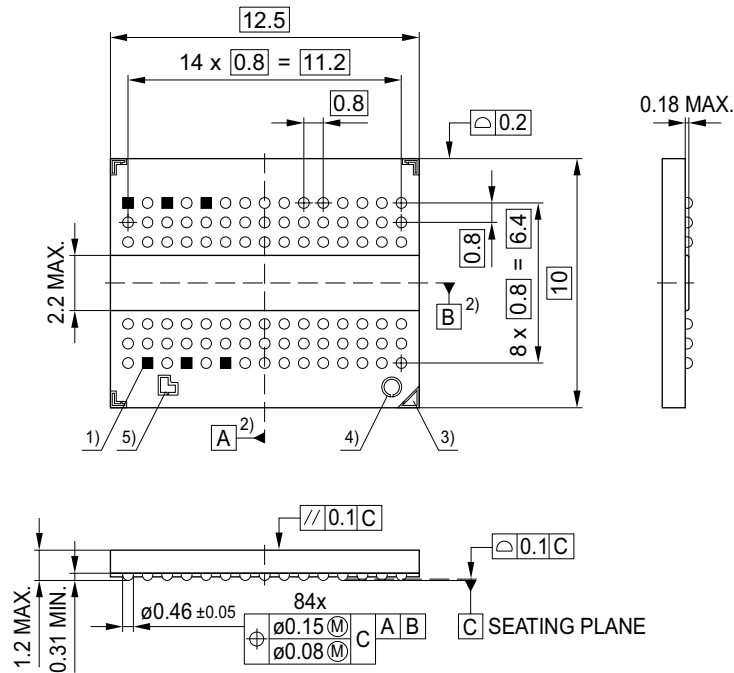
FIGURE 12 Package Outline PG-TFBGA-84
