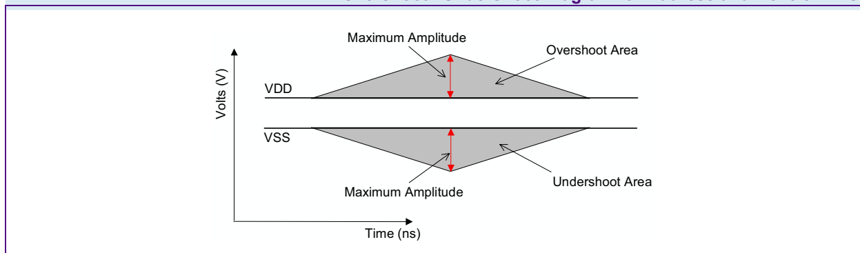
FIGURE 6 AC Overshoot / Undershoot Diagram for Address and Control Pins
