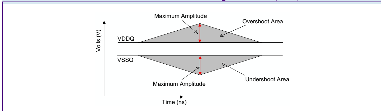
FIGURE 7 AC Overshoot / Undershoot Diagram for Clock, Data, Strobe and Mask Pins
