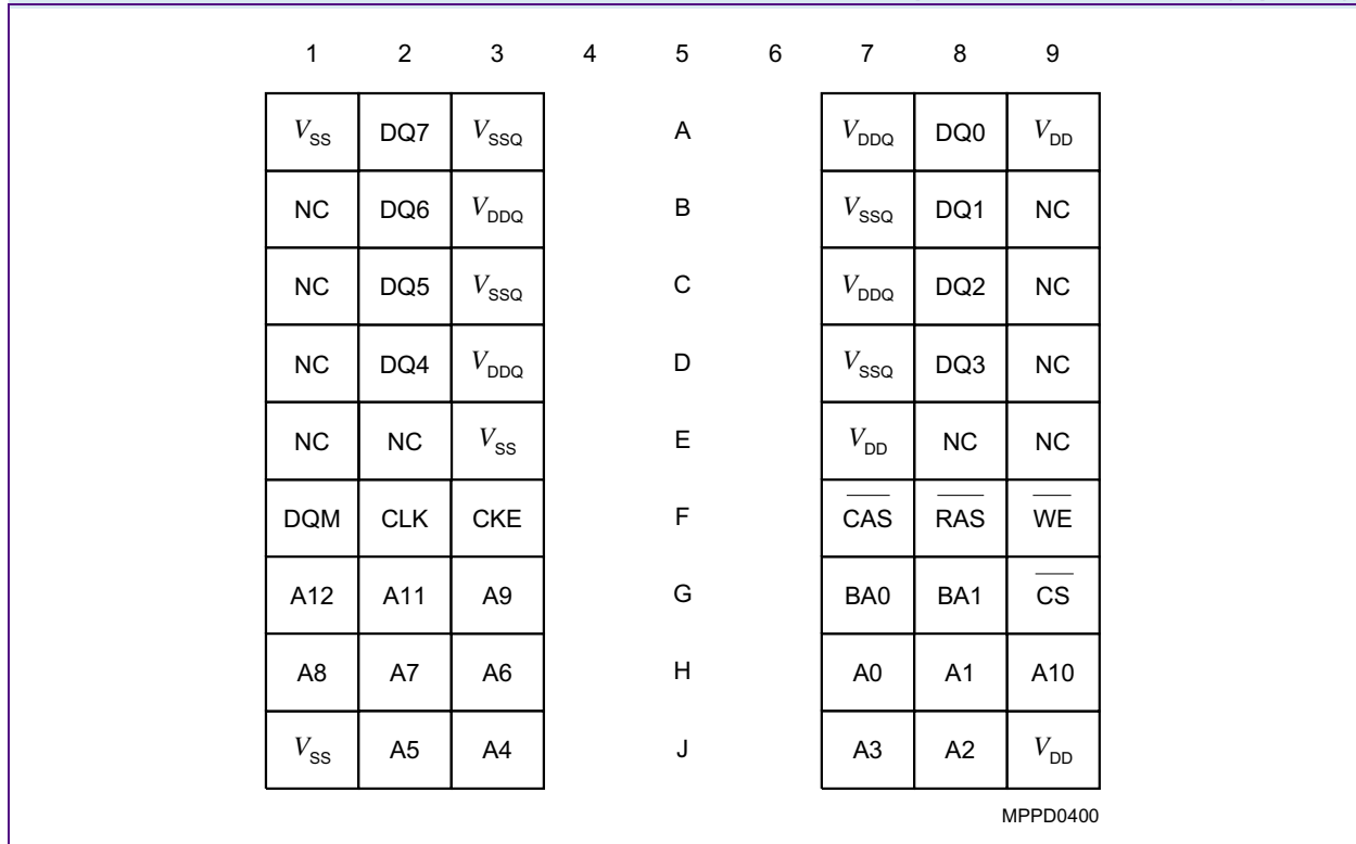
Ballout for ×8 components, PG-TFBGA-54 (top view)
