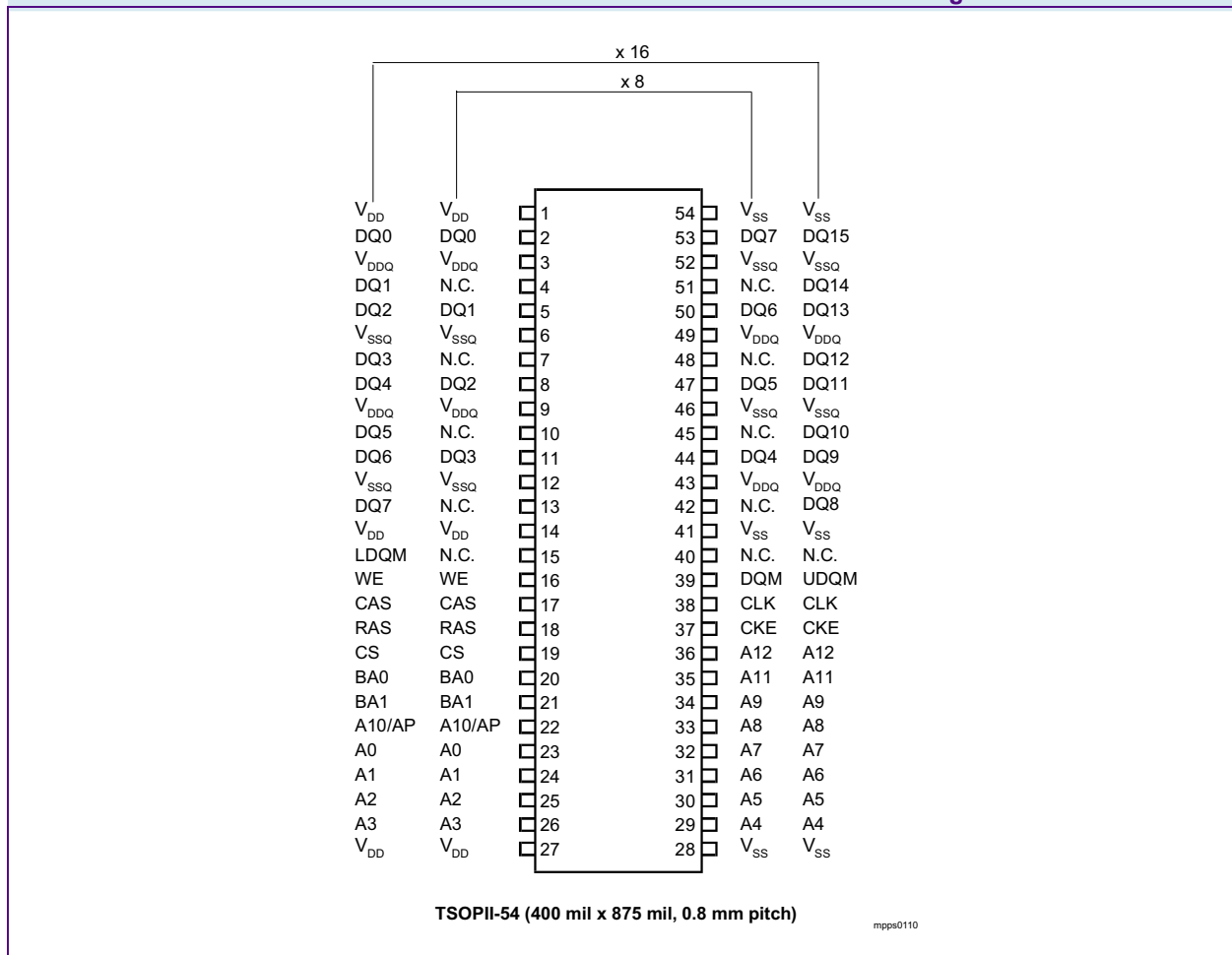
FIGURE 1 Pin Configuration PG-TSOPII-54
