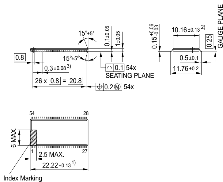
FIGURE 5 Package Outline PG-TSOPII-54 (top view)
