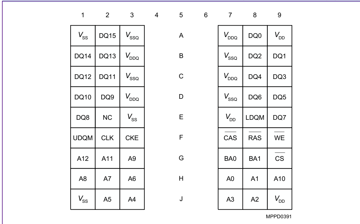
Ballout for ×16 Components, PG-TFBGA-54 (top view)
