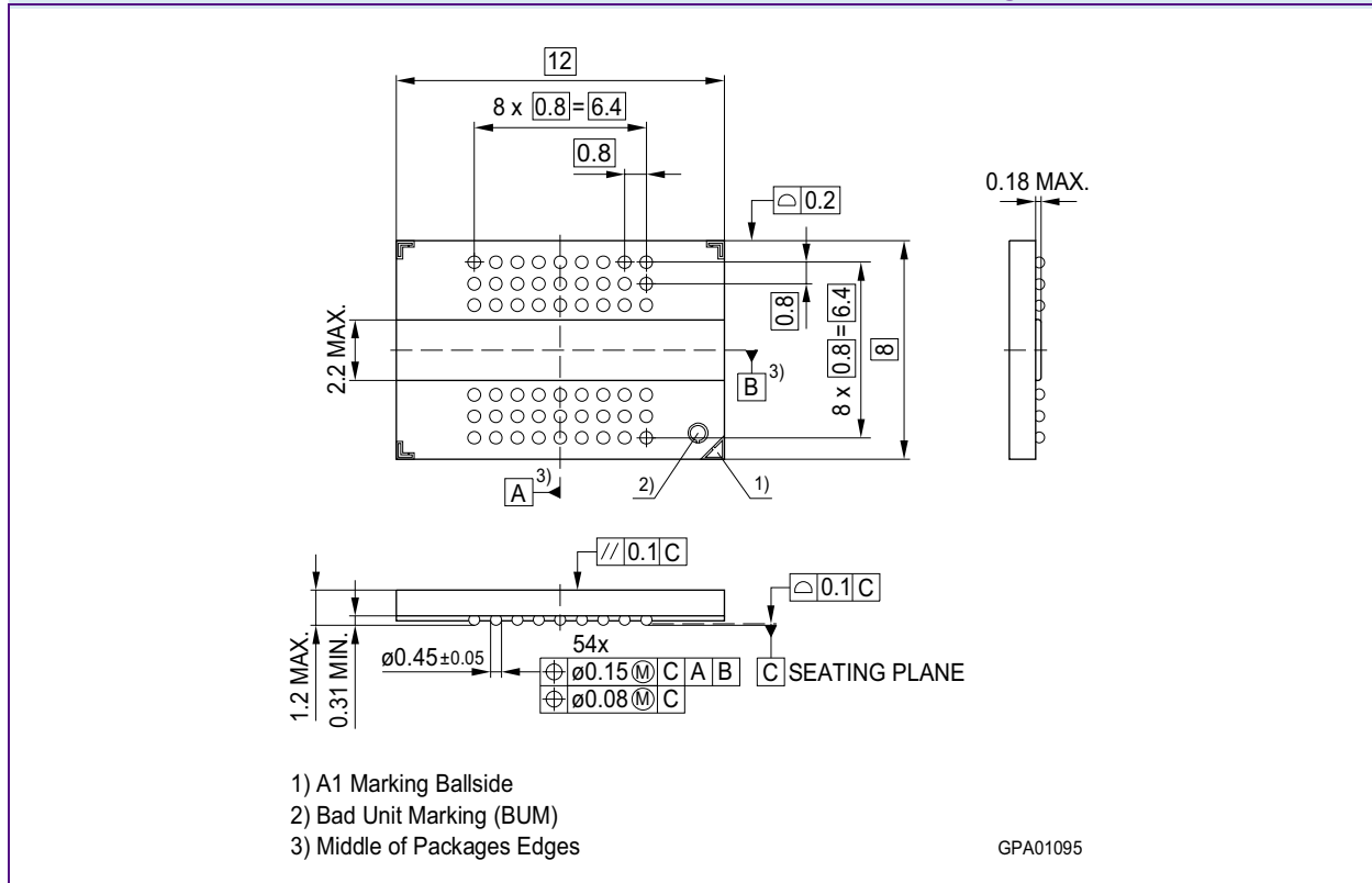
FIGURE 6 Package Outline PG-TFBGA-54-15
