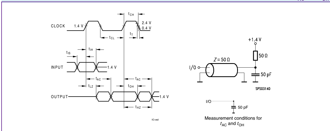
FIGURE 4 Measurement conditions for t_{AC} and t_{OH}
