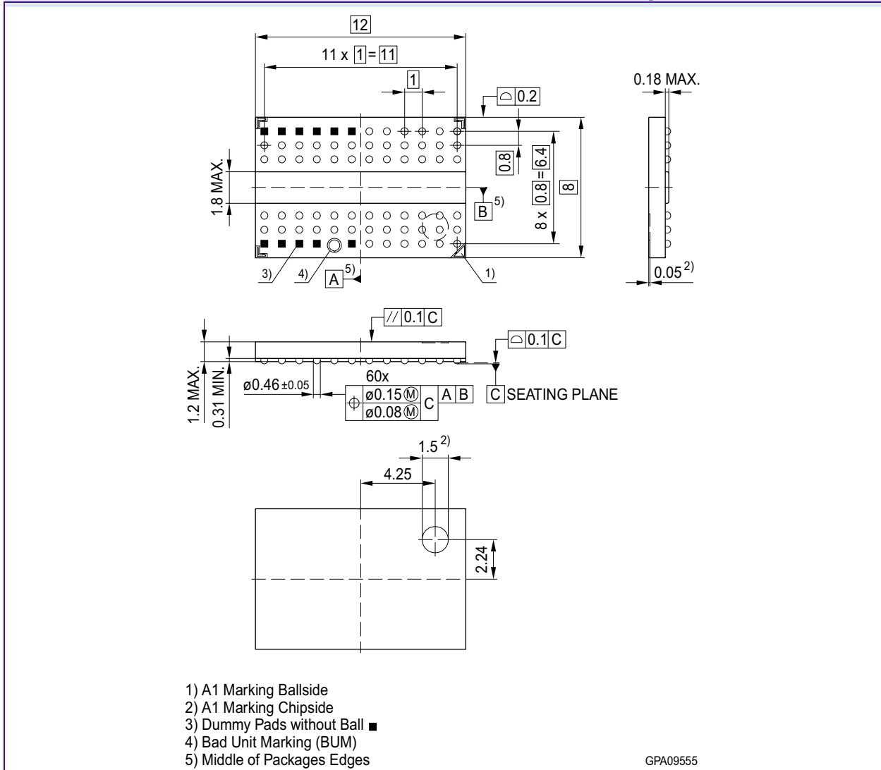
FIGURE 5 Package Outline of PG-TFBGA-60
