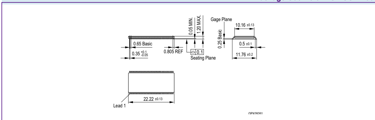
FIGURE 4 Package Outline of PG-TSOPII-66
