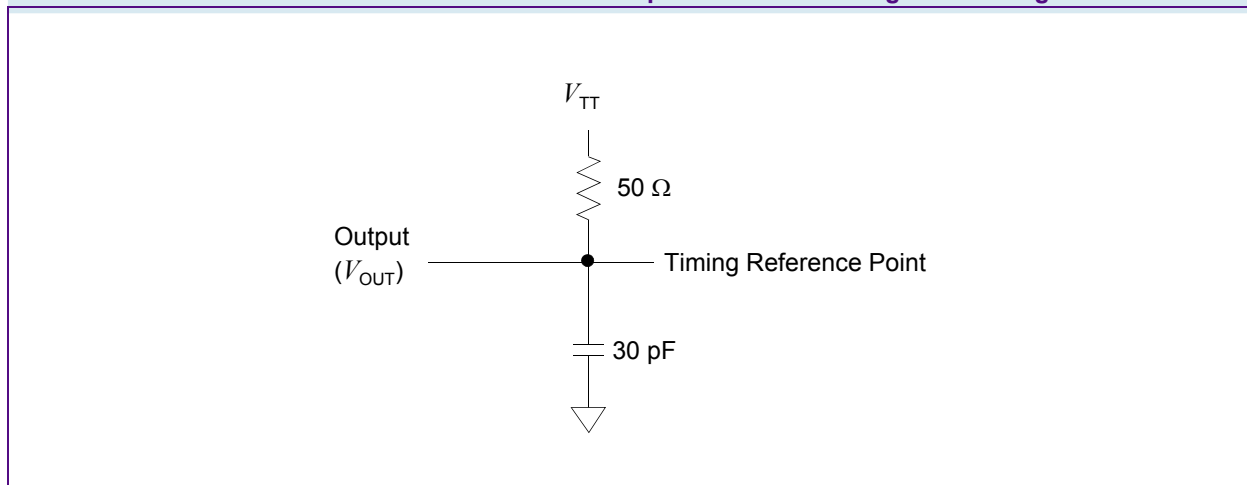
FIGURE 3 AC Output Load Circuit Diagram / Timing Reference Load
