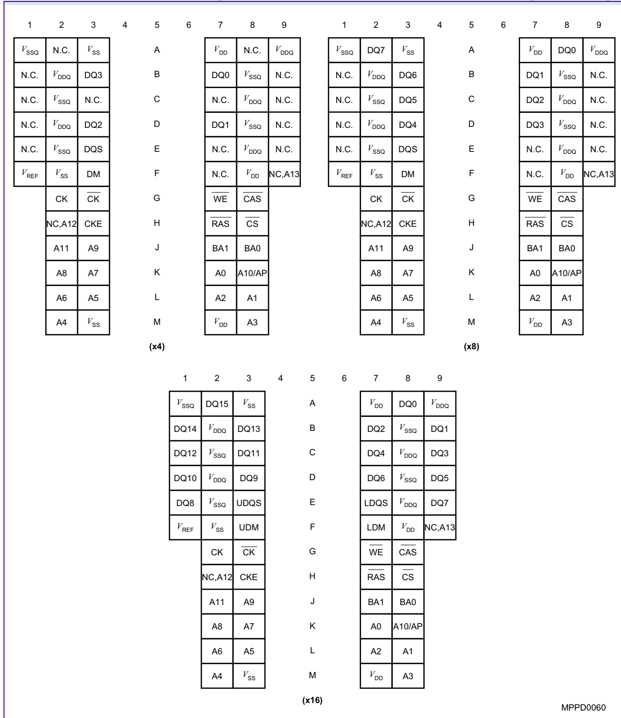
Pin Configuration PG-TFBGA-60 Top View, see the balls through the package
