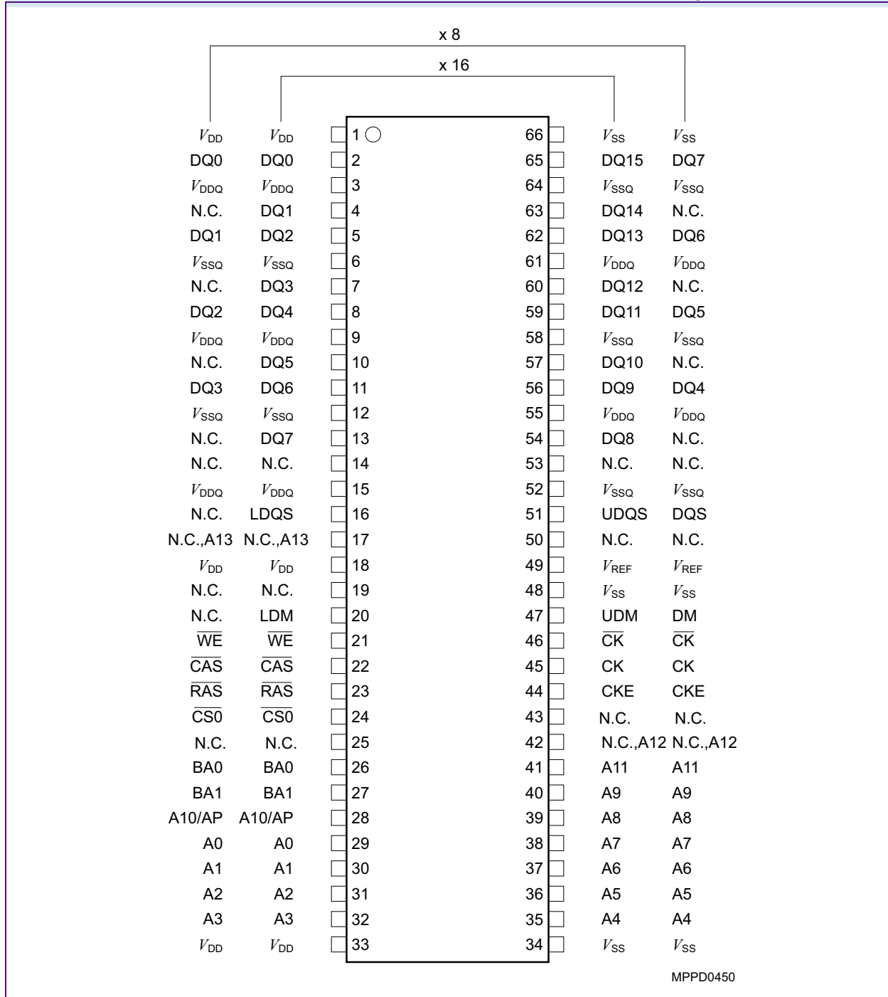
FIGURE 2 Pin Configuration PG-TSOPII-66
