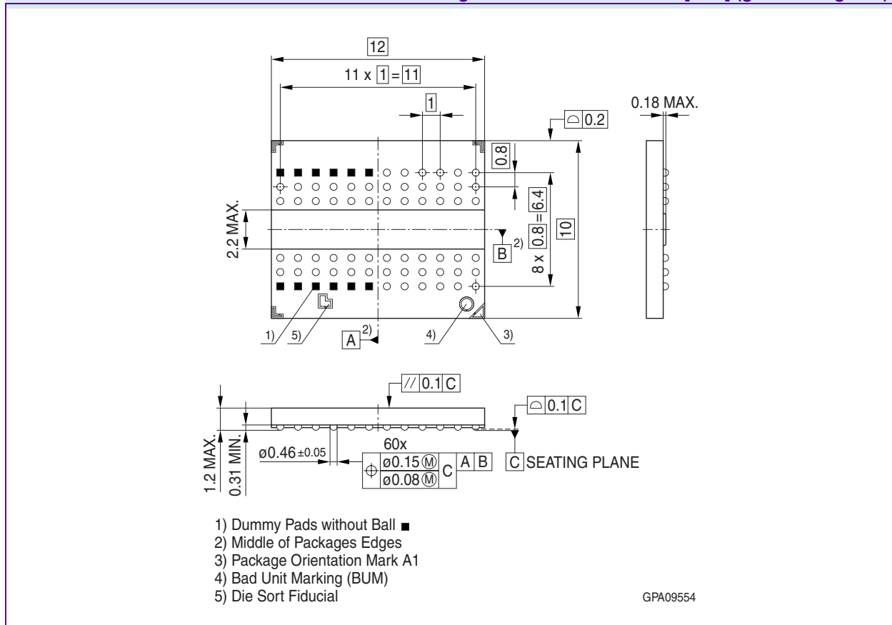
Package Outline of P-TFBGA-60-[9/22] (green/non-green)
