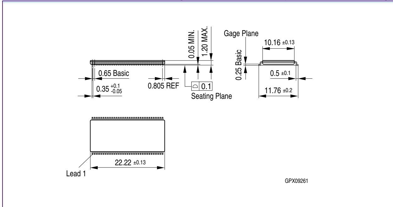
FIGURE 5 Package Outline of P-TSOPII-66-1 (Lead-Free/Lead-Containing)
