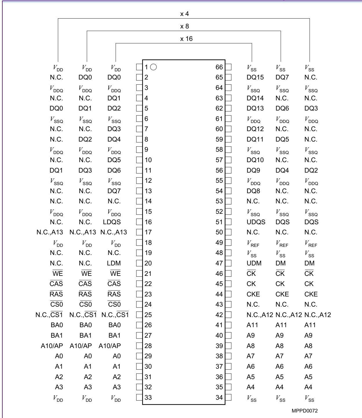
Pin Configuration P-TSOPII-66-1
