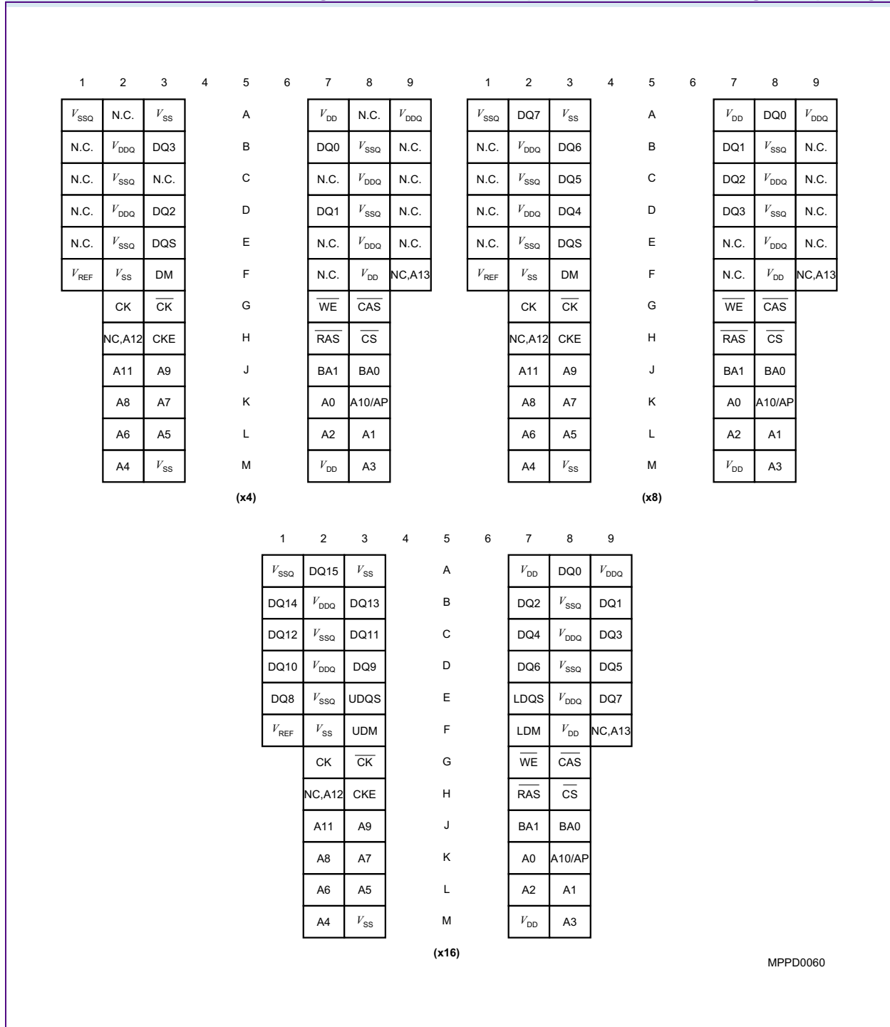
Pin Configuration P-TFBGA-60 Top View, see the balls through the package
