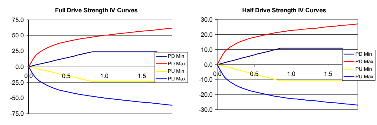
Figure 4 Full Drive Strength and Half Drive Strength
