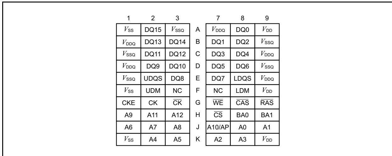
Figure 1 Standard Ballout 512-Mbit DDR Mobile-RAM (Top View)
