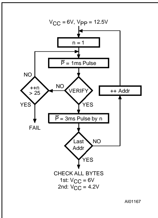
Figure 7. Programming Flowchart
