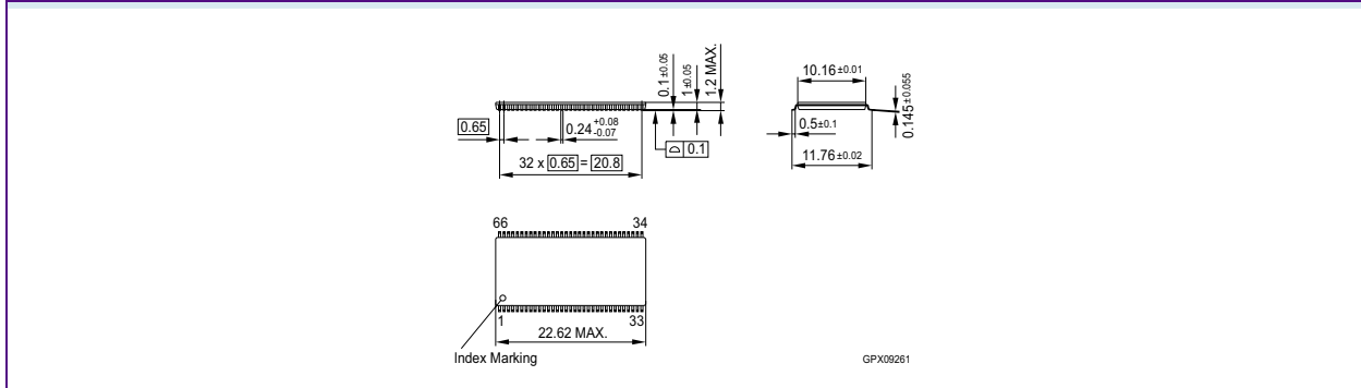
FIGURE 5 Package Outline of P-TSOPII-66-1 (non-green/green)
