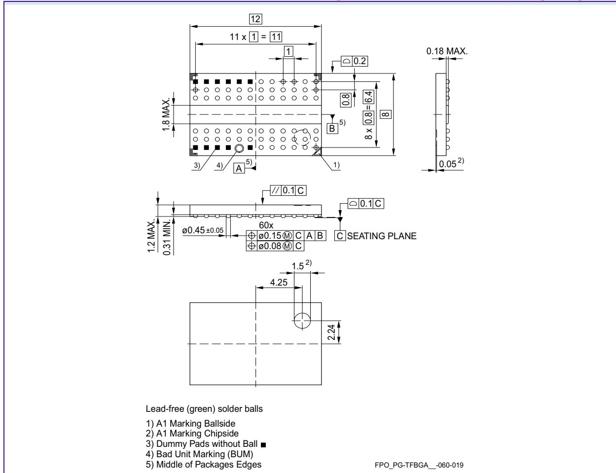
Package Outline of P-TFBGA-60-12 (non-green/green)
