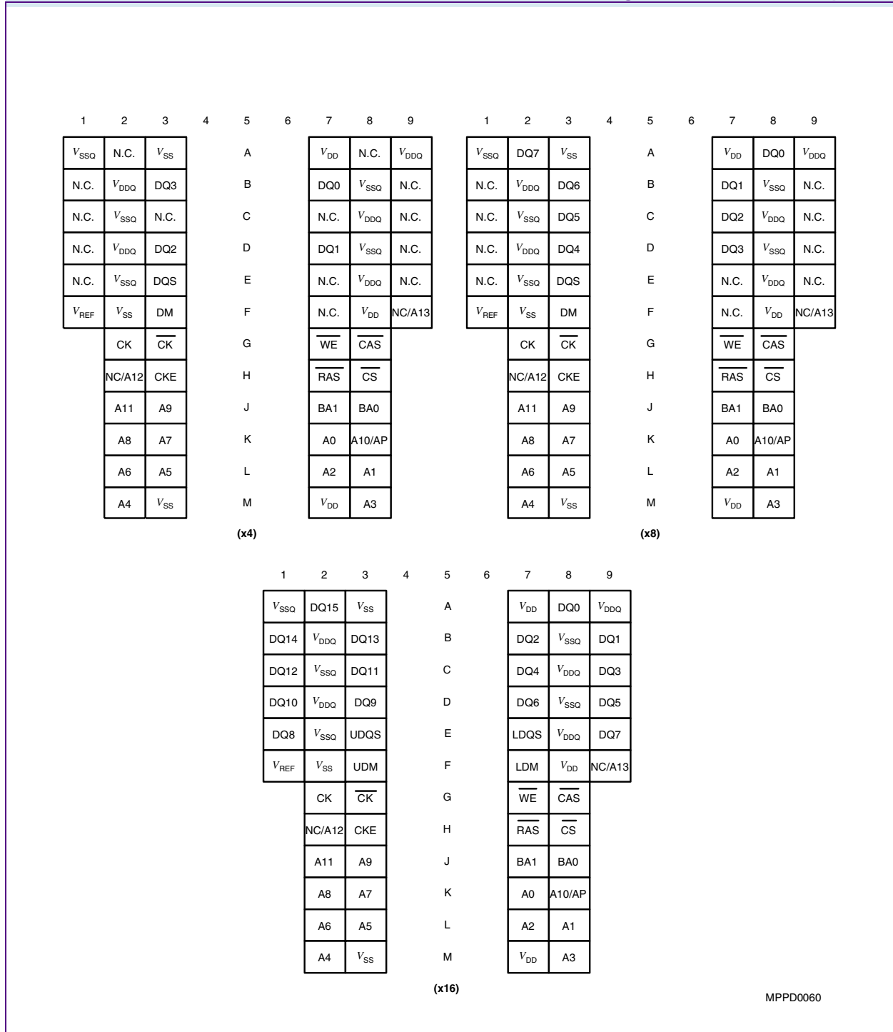
FIGURE 1 Pin Configuration P-TFBGA-60 Top View
