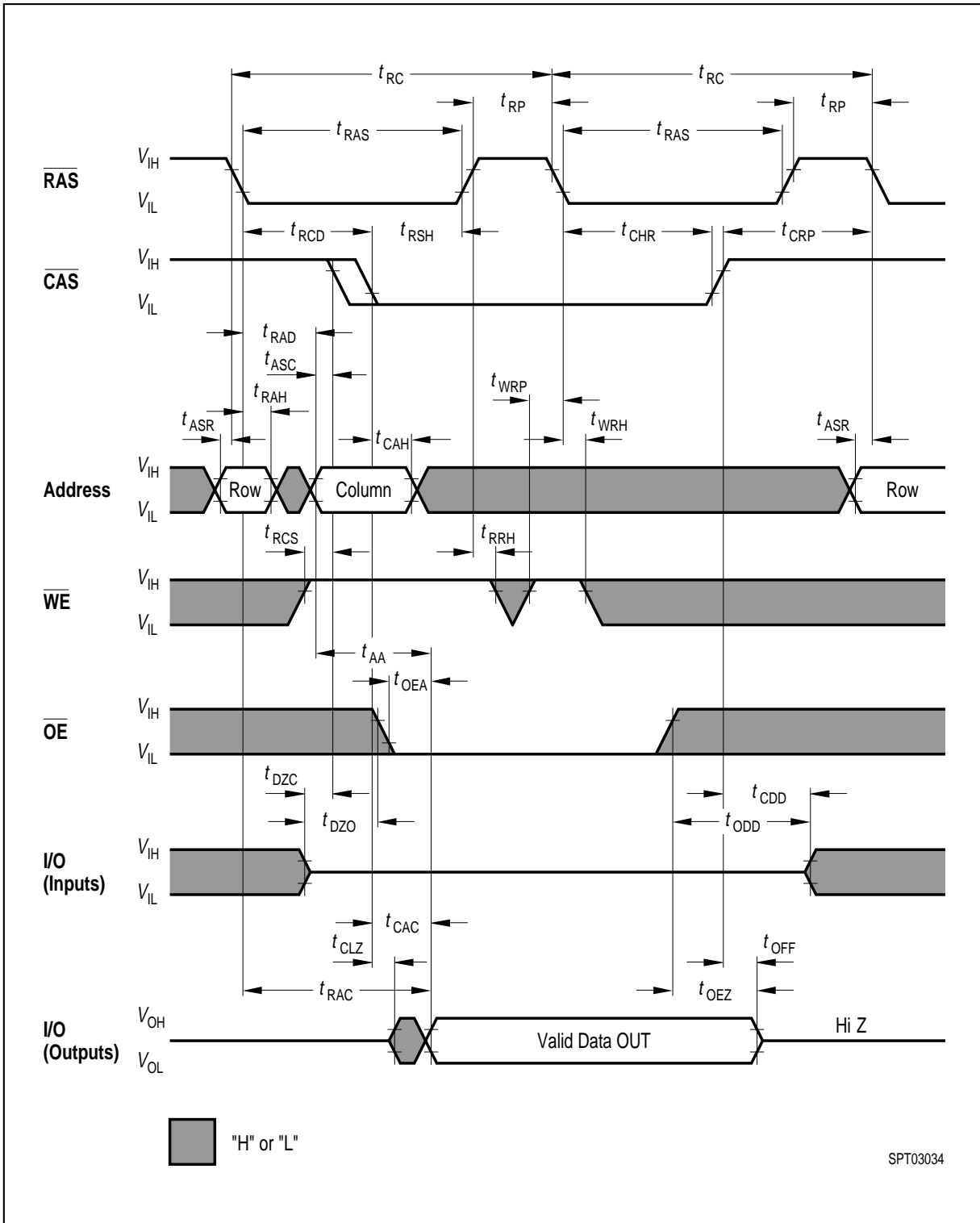
Hidden Refresh Cycle (Read)
