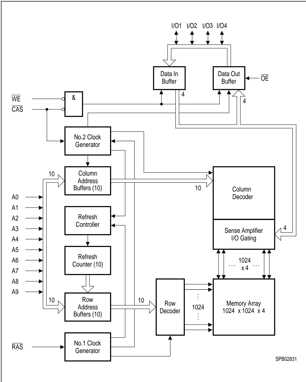
Block Diagram
