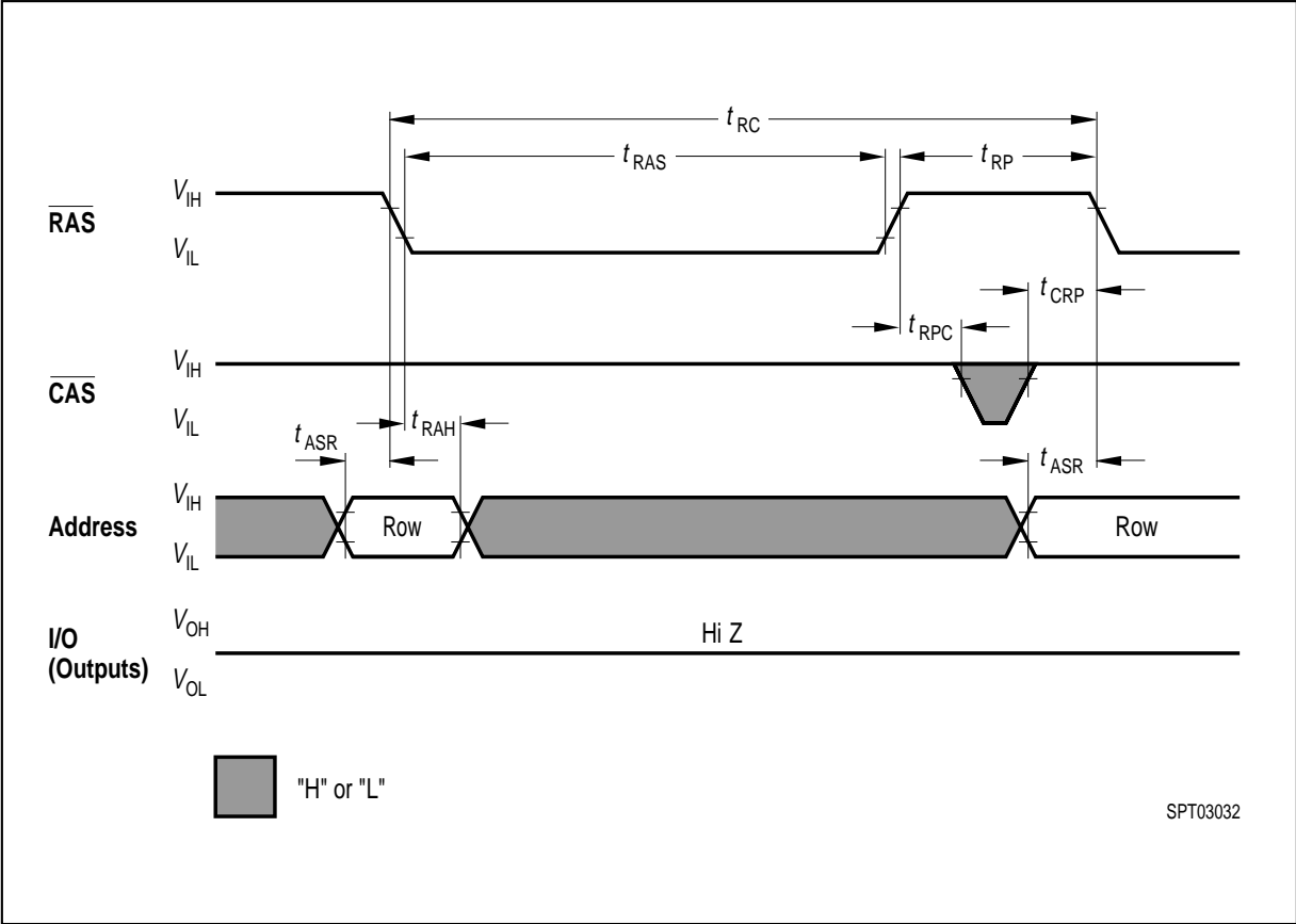
RAS-Only Refresh Cycle
