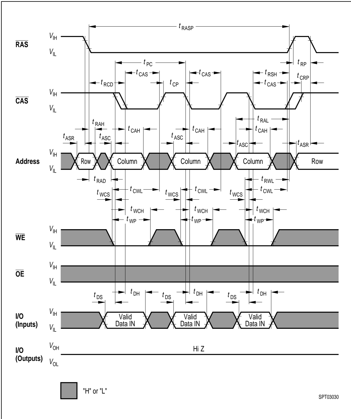
Fast Page Mode Early Write Cycle
