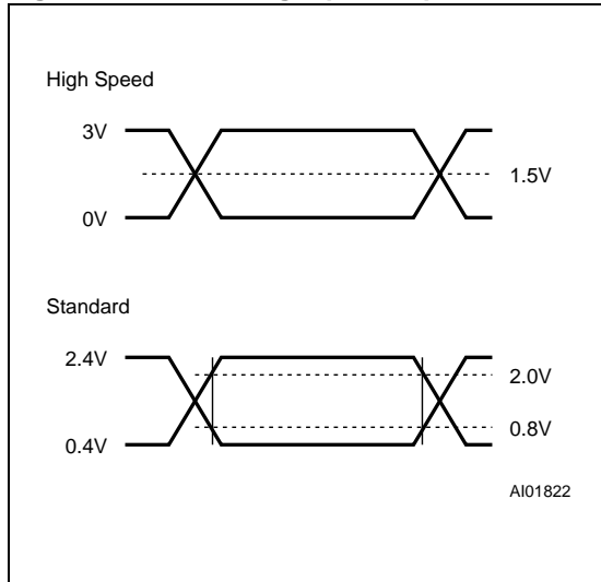
Figure 3A. AC Testing Input Output Waveform
