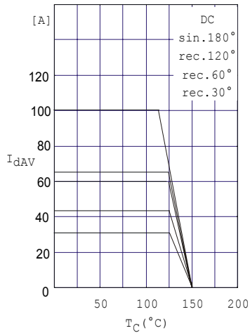
Maximum forward current at case temperature
