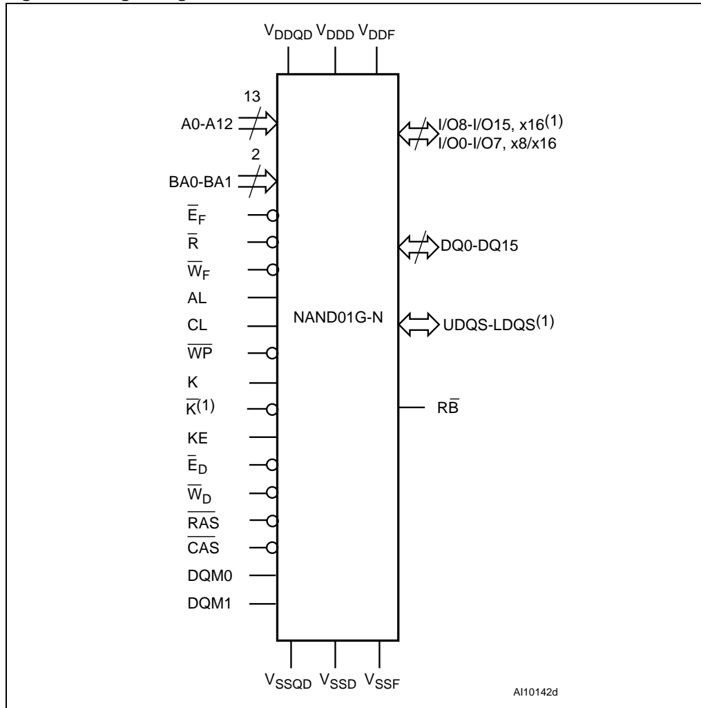
Figure 1. Logic Diagram
