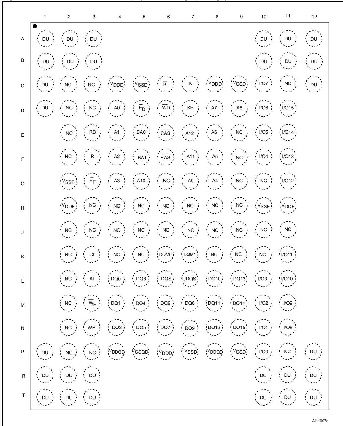
Figure 3. TFBGA149 Connections (Top view through package)
