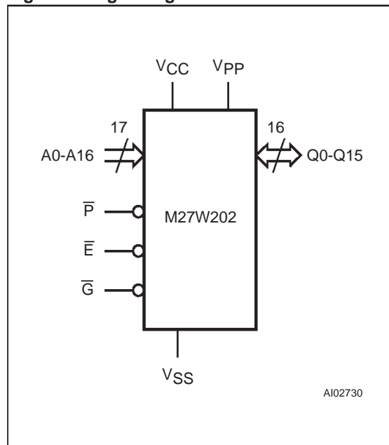
Figure 1. Logic Diagram
