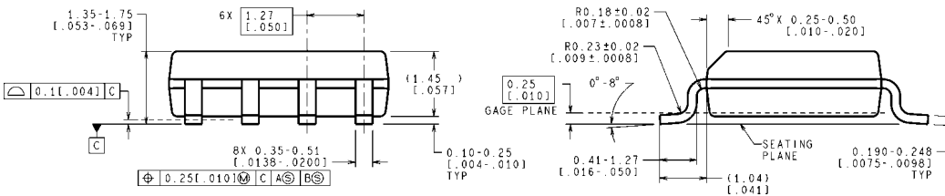
8 Lead Small Outline Molded Package (M) NS Package Number M08A
