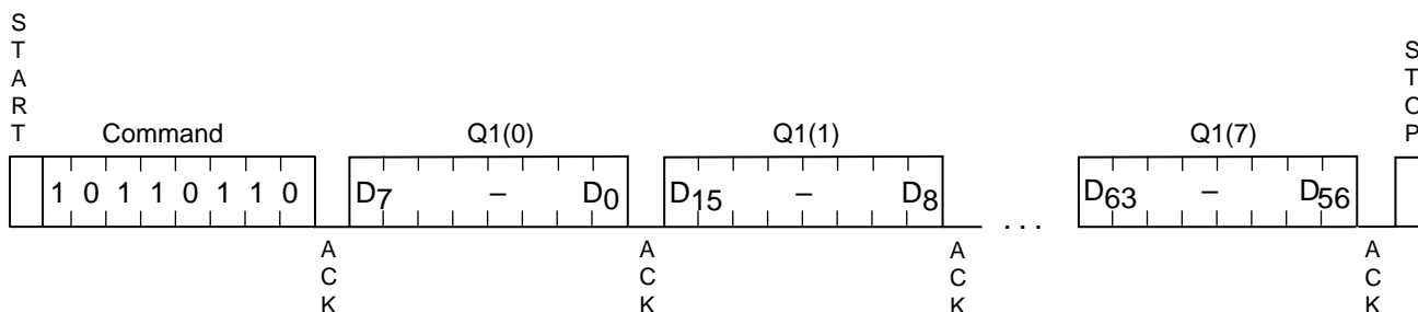
Figure 12. Verify Authentication
