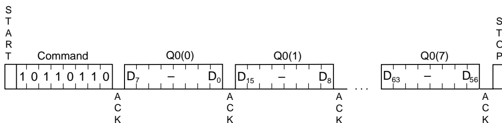
Figure 11. Initialize Authentication
