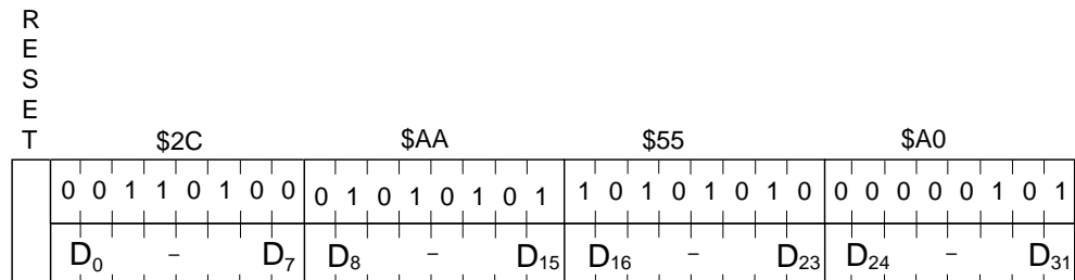
Figure 9. Answer-to-reset
