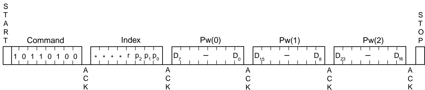
Figure 10. Verify Password
