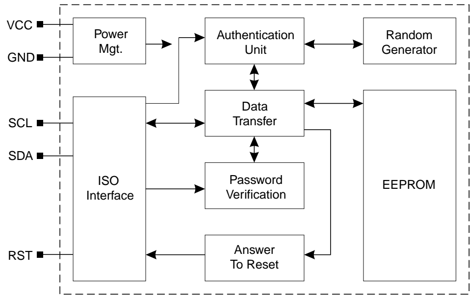
Figure 3. Block Diagram
