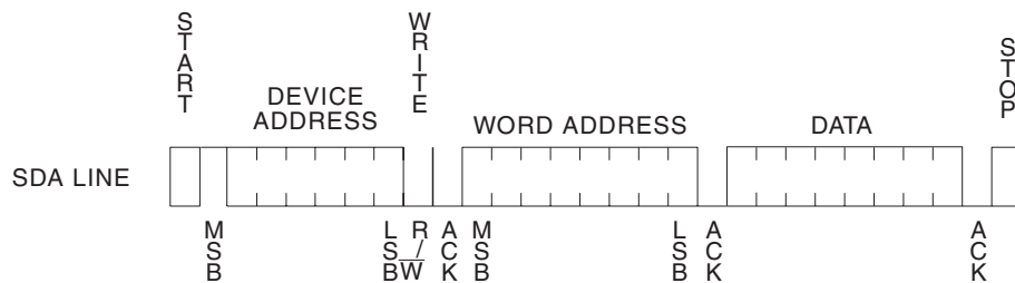
Figure 8. Byte Write
