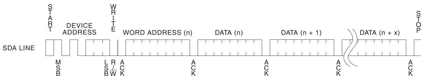
Figure 9. Page Write
