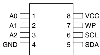
8-lead PDIP
