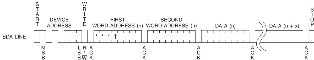
Figure 9. Page Write
