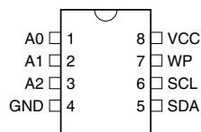
8-lead TSSOP
