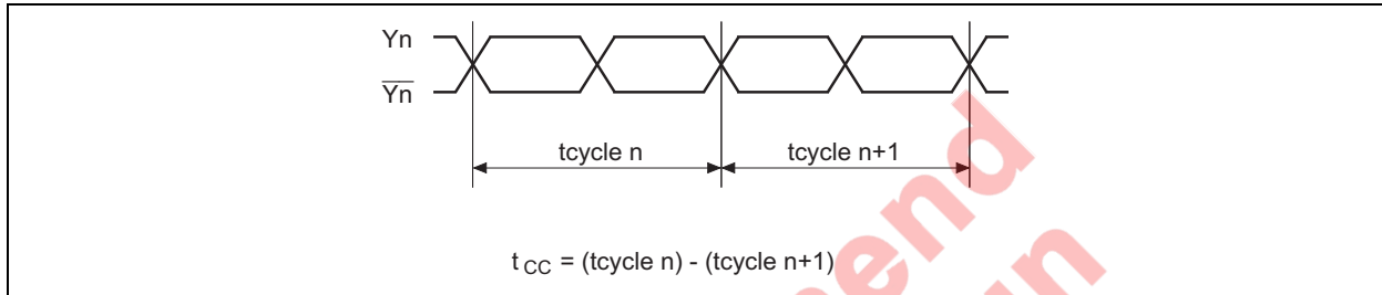
Figure 2 Cycle to cycle jitter
