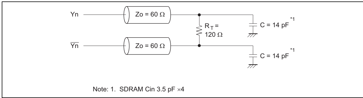
Figure 1 Clock outputs test circuit
