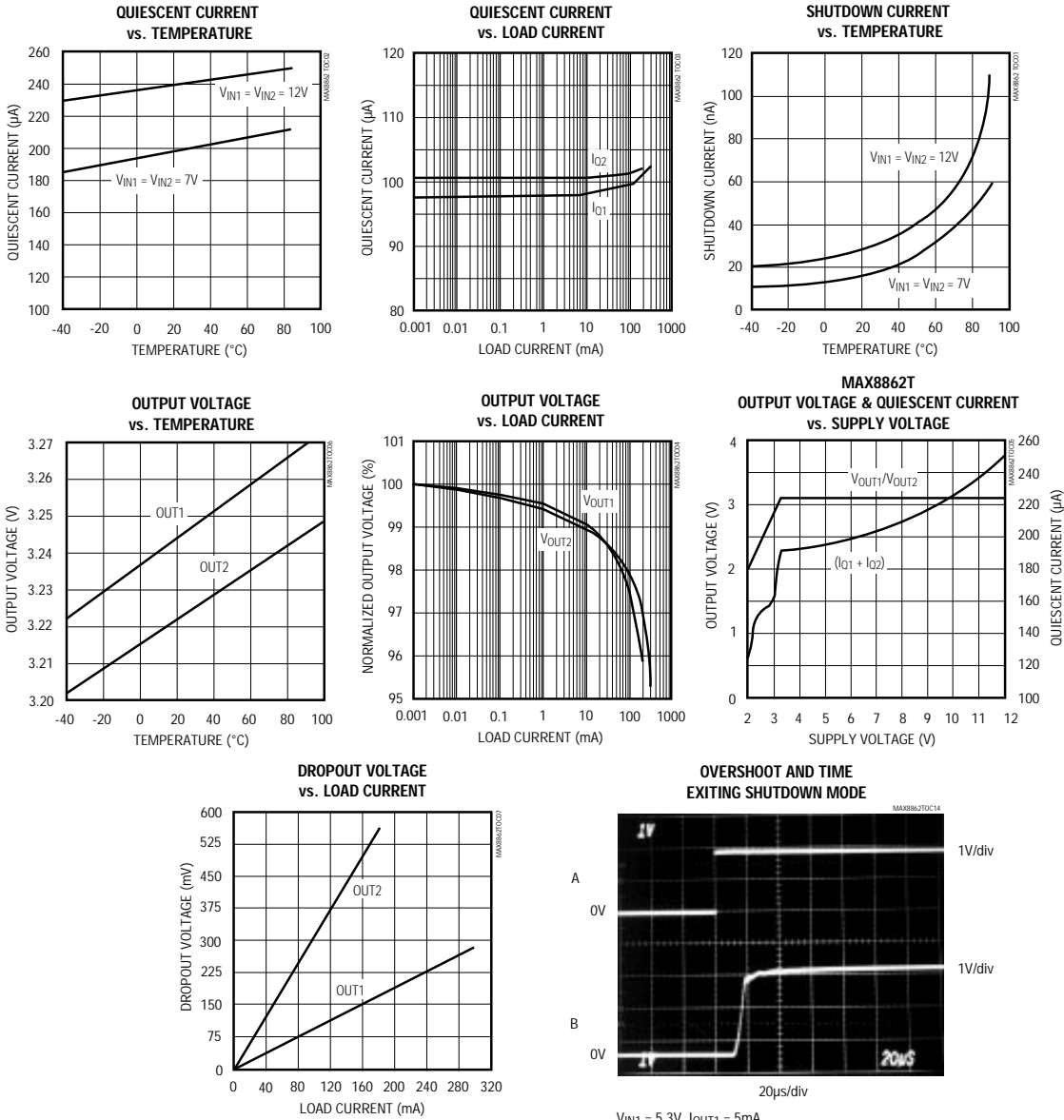
V_{IN1} = 5.3V , I_{OUT1} = 5mA A = SHDN1, 0.8V TO 2.4V, 1V/div B = OUT1, 1V/div
