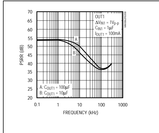
Figure 5b. Power-Supply Rejection Ratio vs. Ripple Frequency for Various Output Capacitors
