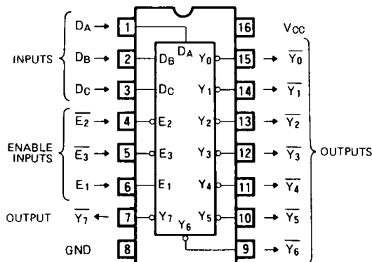
Outline 16P4
