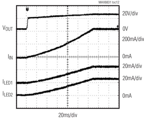
SOFT-START RESPONSE
