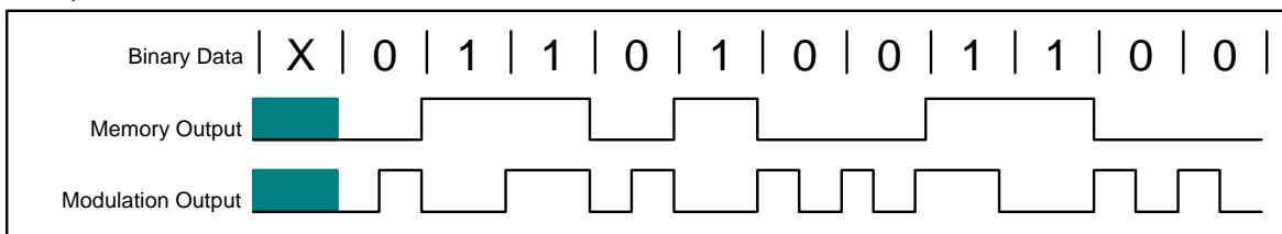
Biphase Code
