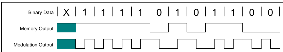
Manchester Code
