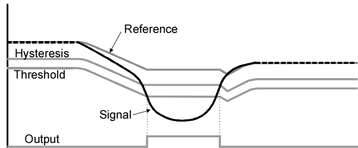
Figure 1-7 Drift Compensation
