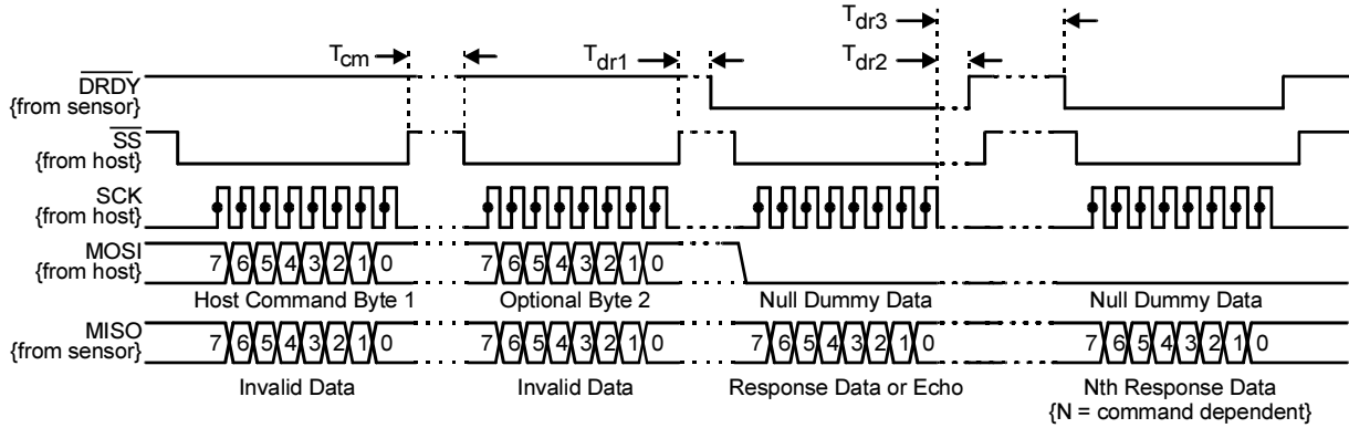
Figure 4-3 SPI Slave-Only Mode Timing
