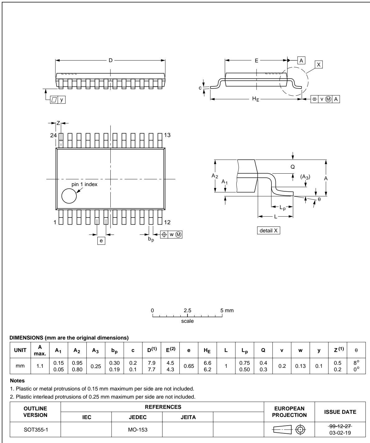
Fig 12. Package outline SOT355-1 (TSSOP24)
